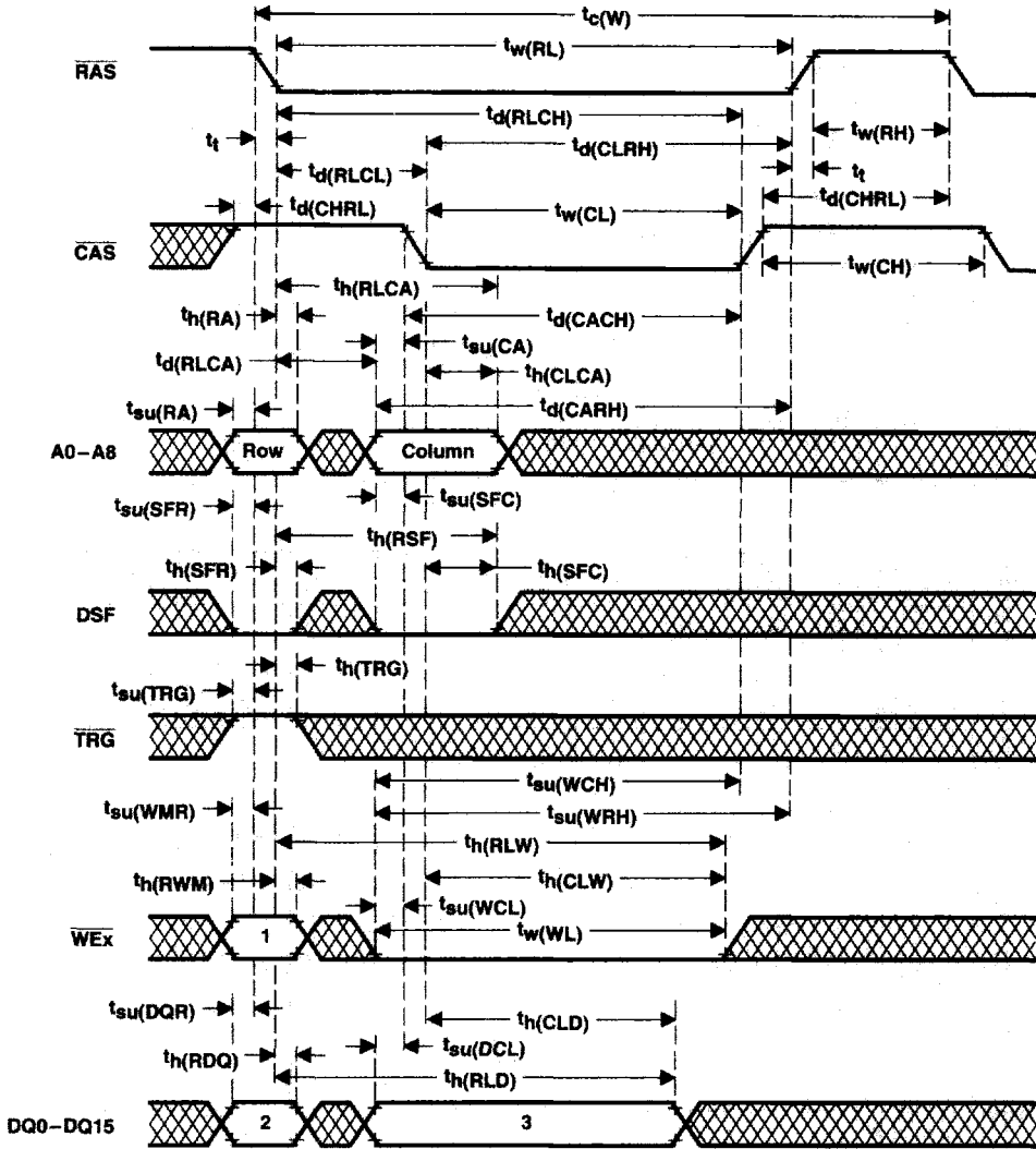
Figure 28. Early-Write-Cycle Timing
