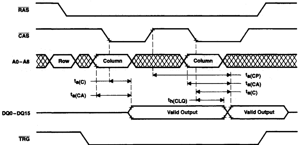
Figure 3. DRAM Page-Read Cycle With Extended Output
