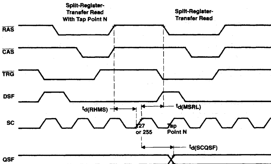
Figure 19. Example of Successive Split-Register-Transfer Read Operations
