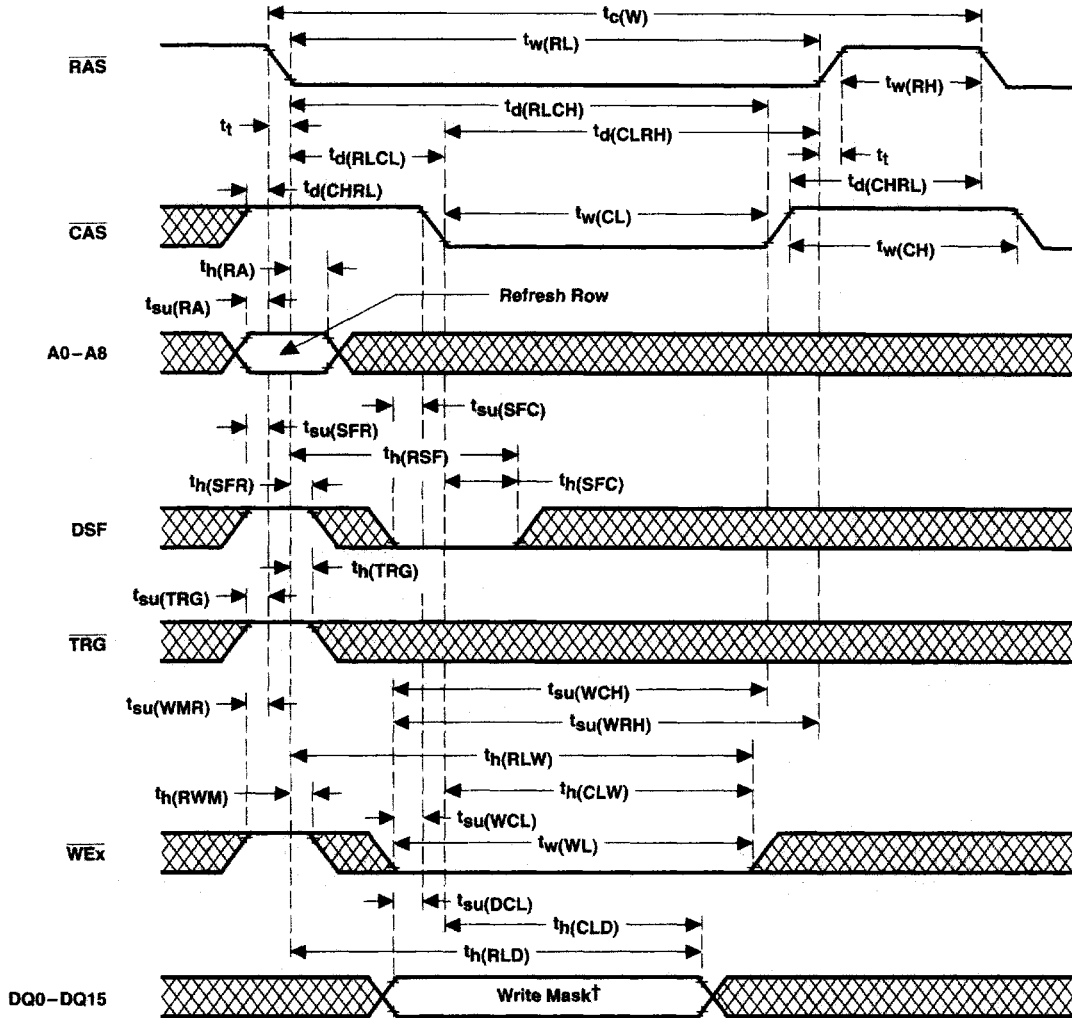
Figure 30. Load-Write-Mask-Register-Cycle Timing (Early-Write Load)
