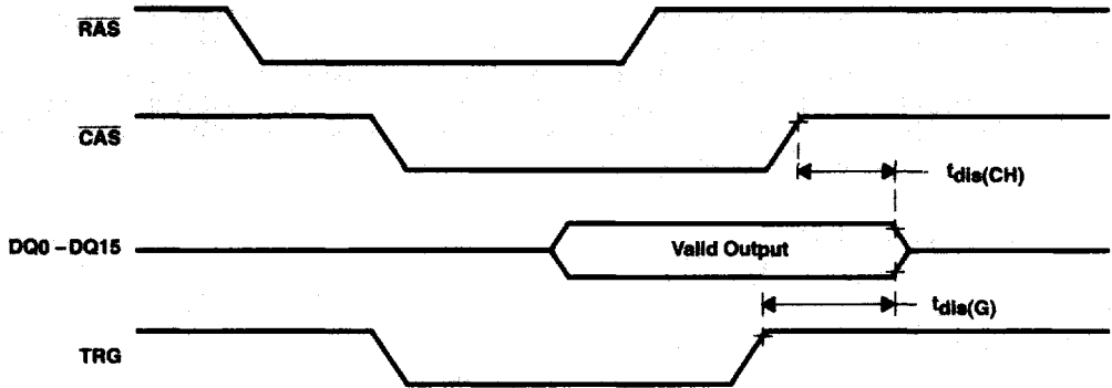
Figure 2. DRAM Read Cycle With \overline{CAS} -Controlled Output
