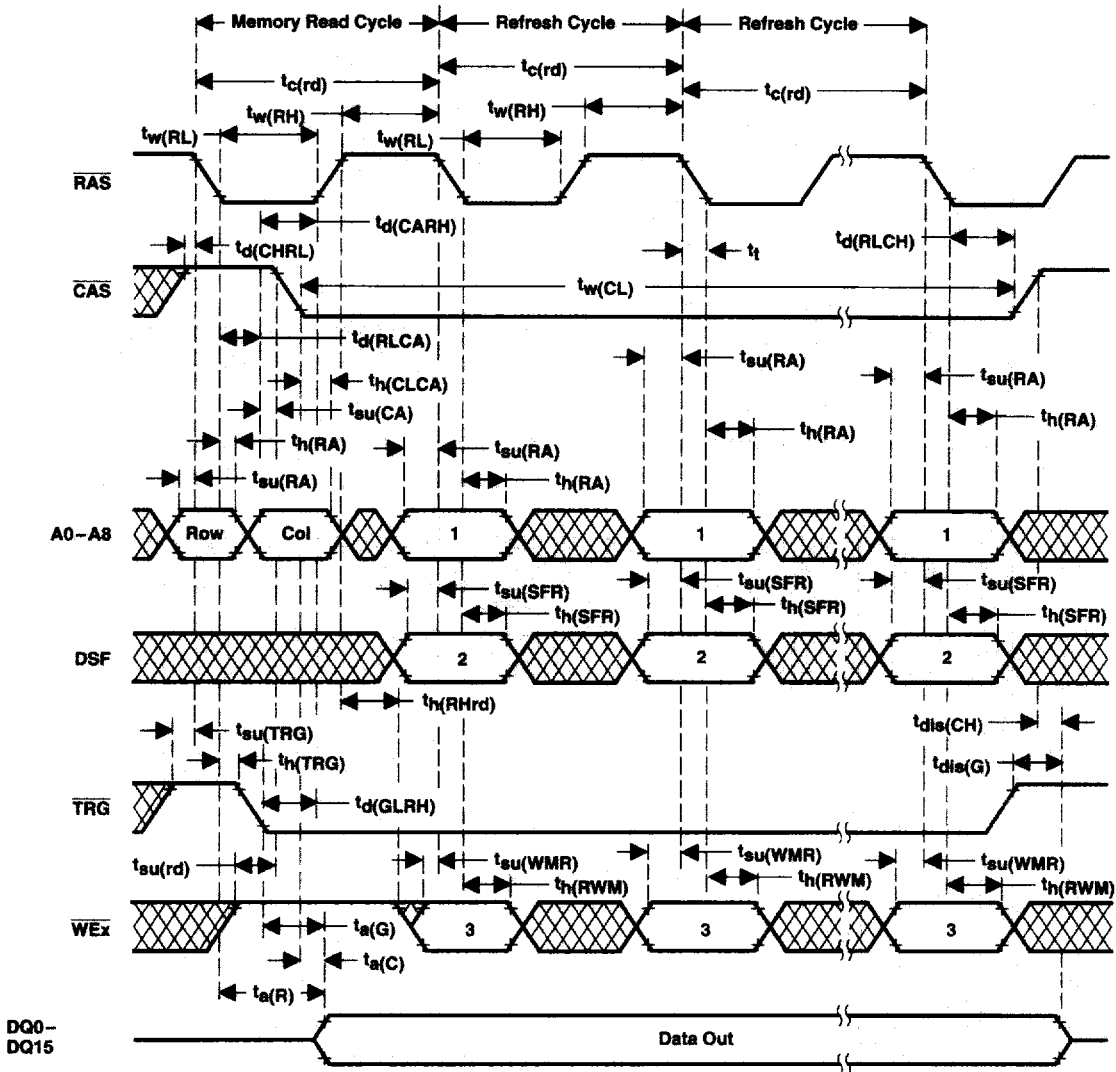
Figure 44. Hidden-Refresh-Cycle Timing
