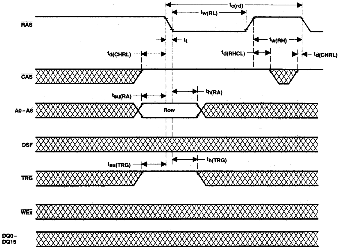
Figure 42. RAS-Only Refresh-Cycle Timing
