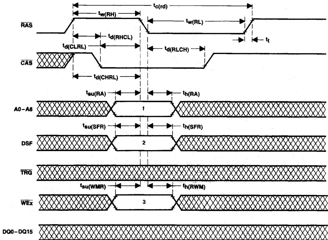
Figure 43. CBR-Refresh-Cycle Timing
