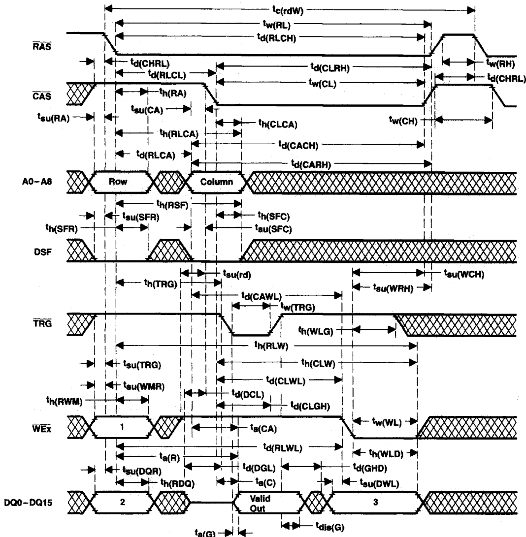
Figure 32. Read-Write-/Read-Modify-Write-Cycle Timing
