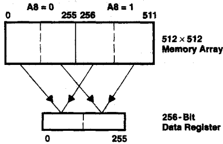
Figure 16. Split-Register-Transfer Read
