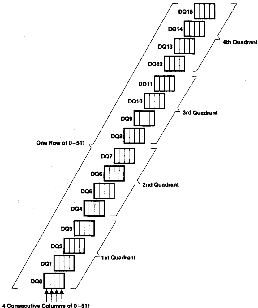
Figure 8. Block-Write Operation
