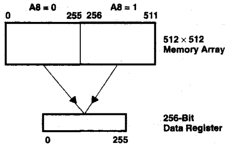
Figure 14. Full-Register-Transfer Read
