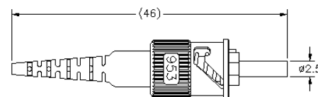
ST II Connector with 900µm Boot
