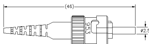
ST Connector with 900µm Boot
