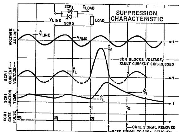
FIG. 1 SUPPRESSION CHARACTERISTICS
