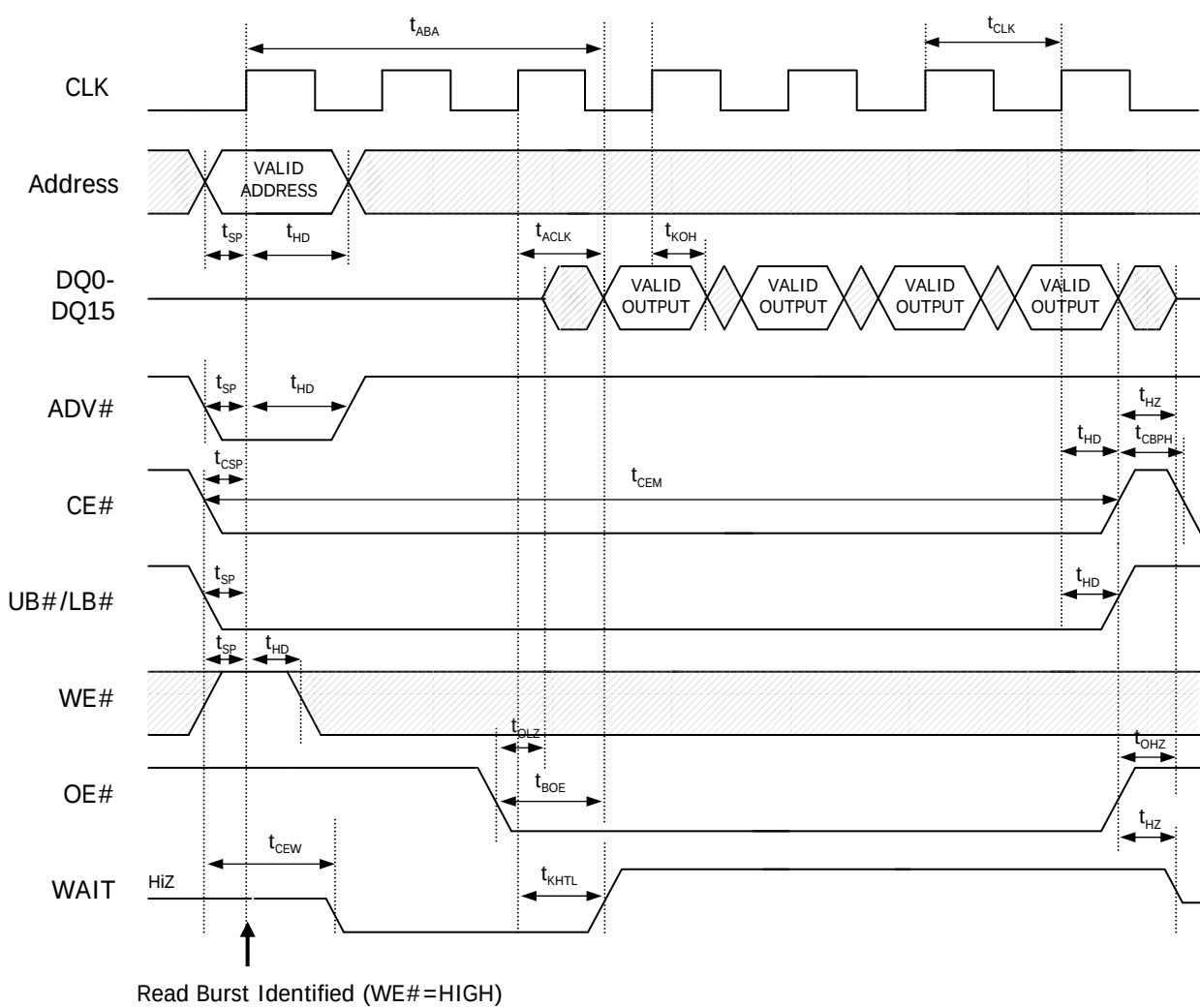
Figure 25: Four-Word Burst READ Operation – Variable Latency without refresh collision
