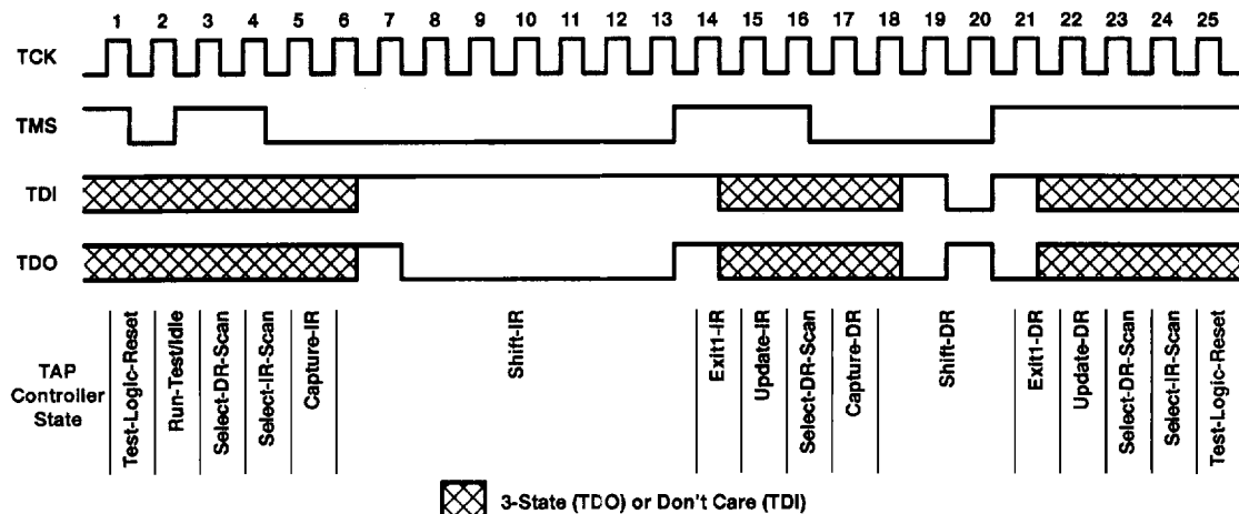
Figure 13. Timing Example
