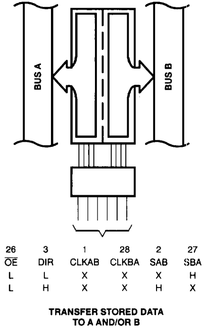
Figure 1. Bus-Management Functions
