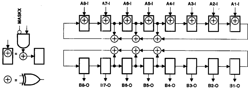
Figure 9. 8-Bit PSA/PRPG Configuration (OEA = 0, OEB = 1)
