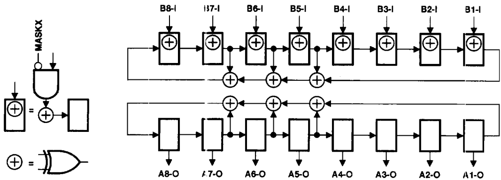
Figure 10. 8-Bit PSA/PRPG Configuration (OEA = 1, OEB = 0)
