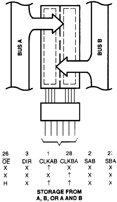
Figure 1. Bus-Management Functions
