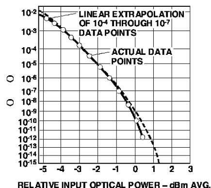
Figure 3. Relative Input Optical Power dBm Average.
