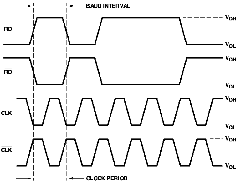
Figure 2. Relative Timing Relationship Between Output Retimed Data and Recovered Clock Signals.
