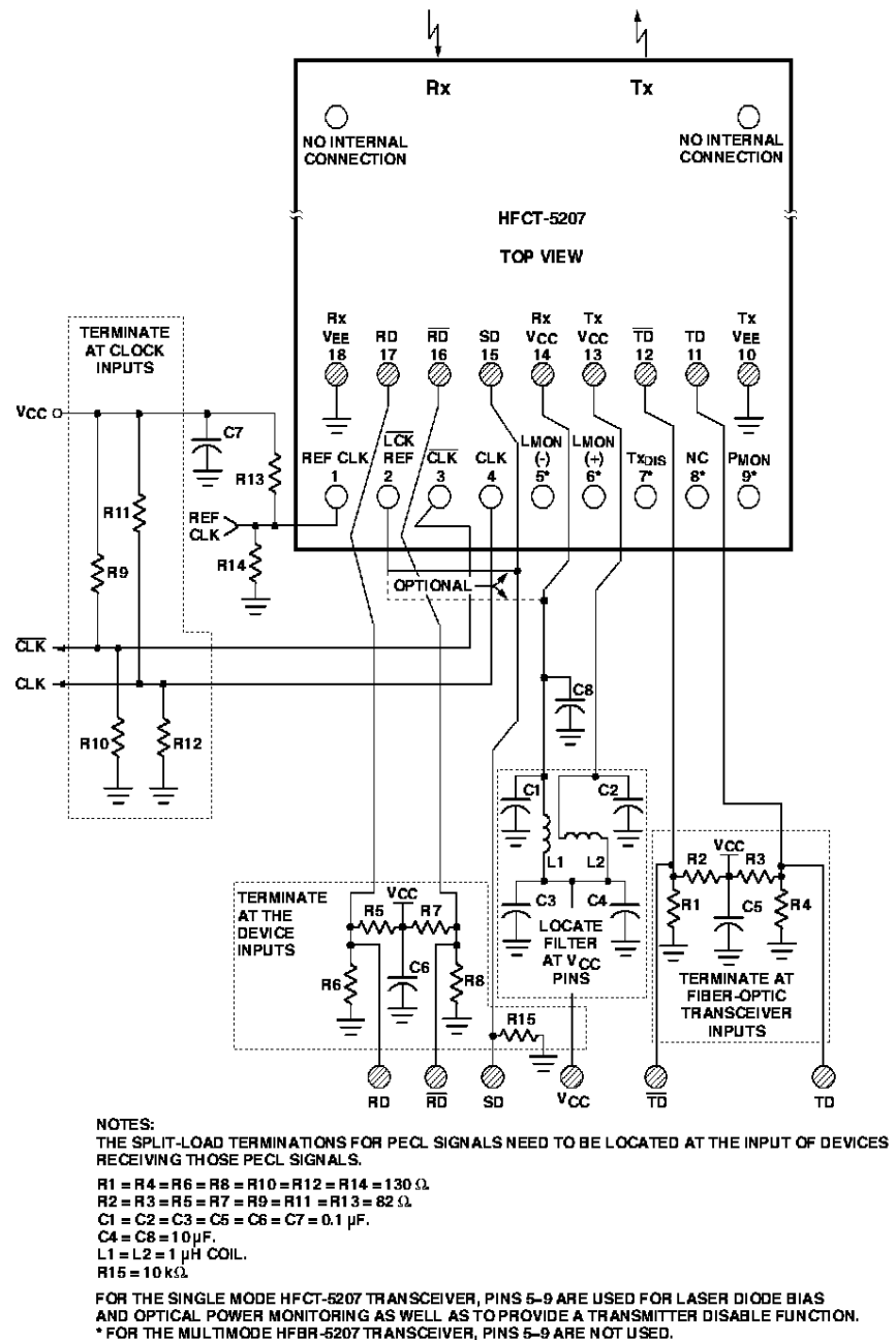
Figure 4. Recommended Circuit Schematic.
