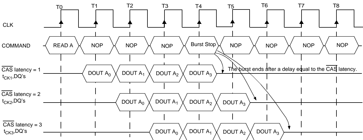
Termination of a Burst Write Operation (Burst Length > 4, \overline{\text{CAS}} Latency = 1, 2, 3)
