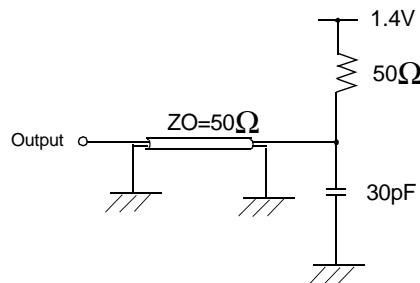
LVTTTL D.C. Test Load (B)
