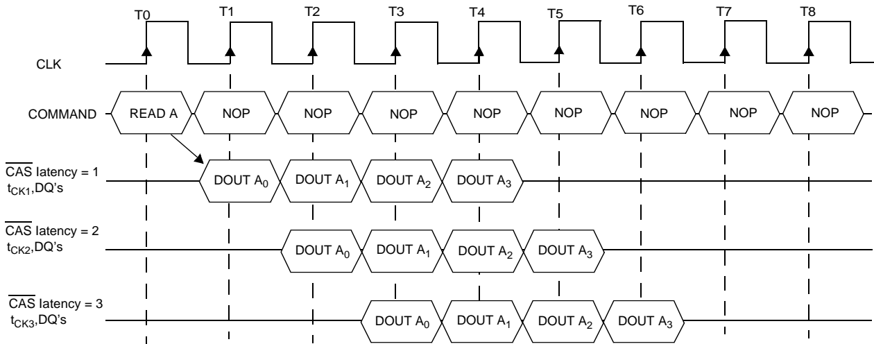
Burst Read Operation (Burst Length = 4, \overline{\text{CAS}} Latency = 1, 2, 3)
