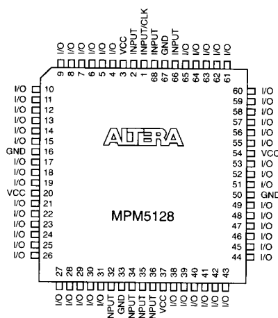
Figure 9. MPM5128 Package Pin-Out Diagram
