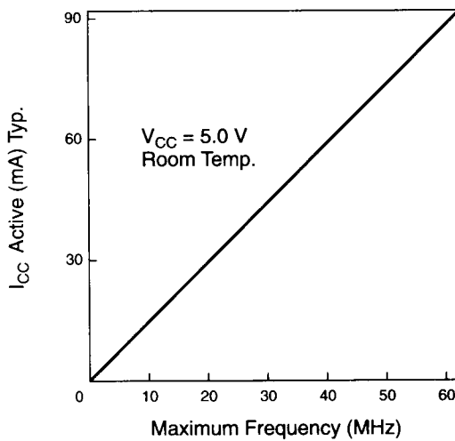
Figure 10. MPM5128 I_{CC} vs. Frequency
