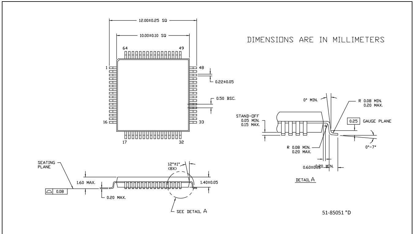
Figure 7 64-pin TQFP (10 × 10 × 1.4 mm) Package Outline, 51-85051
