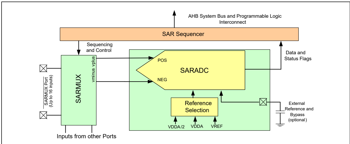
Figure 4 SAR ADC
