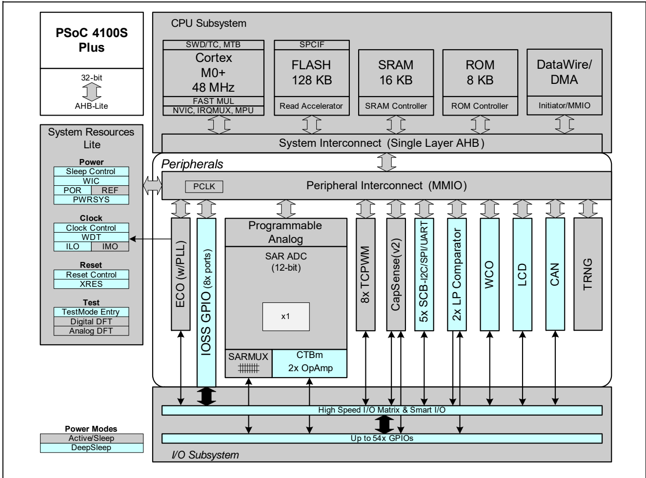
Figure 2 Block diagram
