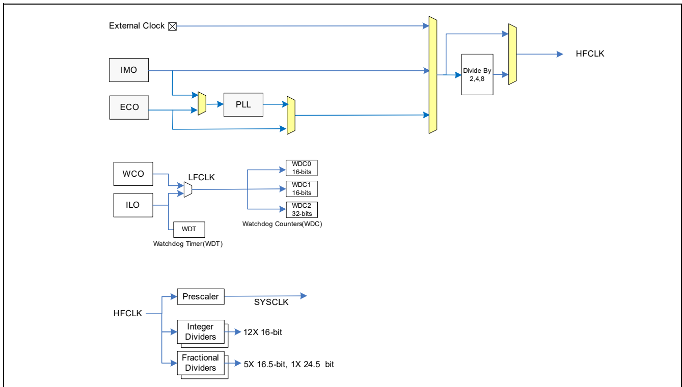
Figure 3 PSoC™ 4100S Plus MCU clocking architecture
