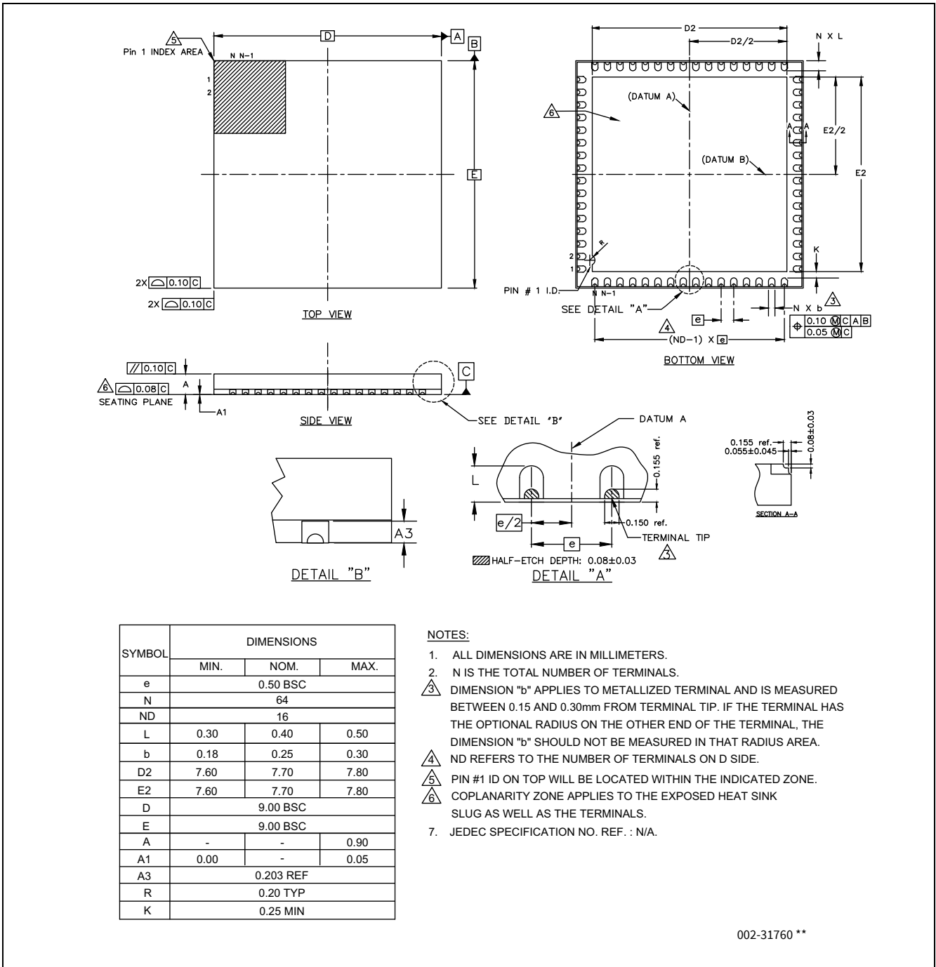
Figure 9 64-pin QFN (9 × 9 × 0.9 mm (7.70 × 7.70 mm E-Pad (Sawn))) Package Outline, 002-31760
