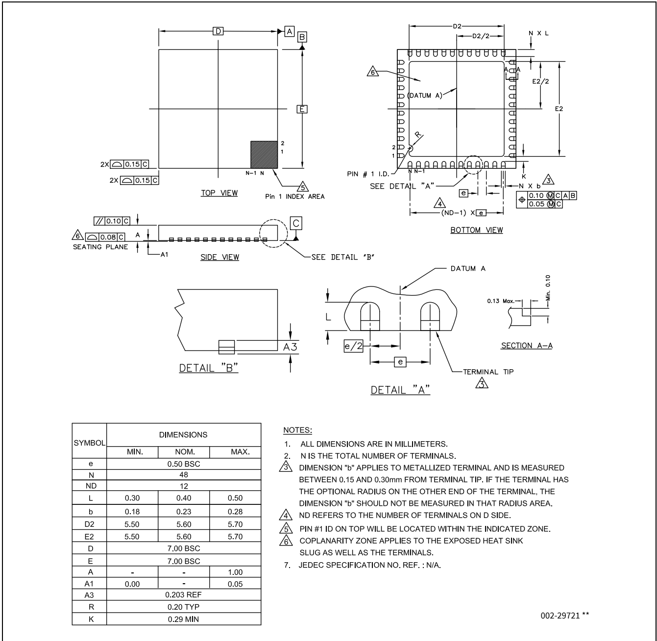
Figure 10 48-pin QFN ( 7 × 7 × 1.0 mm) wettable flank package)
