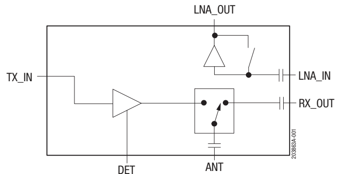
Figure 1. SKY85331-11 Block Diagram
