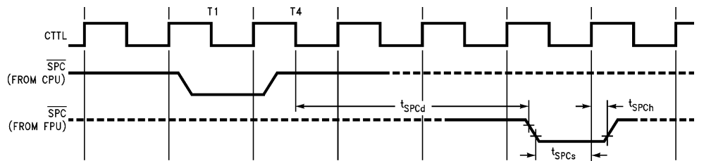
After transferring the last operand to the FPU, the CPU turns OFF the output driver and holds \overline{\text{SPC}} high with an internal 5 k \Omega pullup. FIGURE 4-12. \overline{\text{SPC}} Timing TL/EE/11267-54
