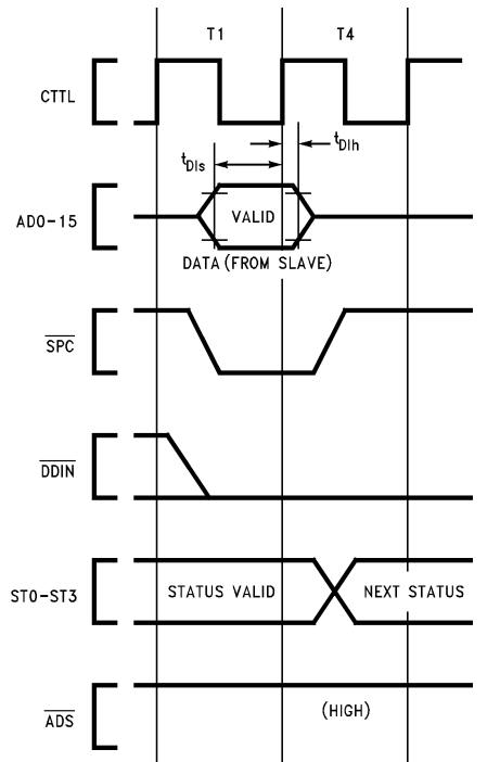
FIGURE 4-11. Slave Processor Read Timing TL/EE/11267-53
