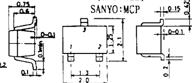
Case Outlines (unit:mm)
