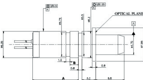
SC TOSA (L&M Power with Isolator) C-13-DFB2.5-TX-SSCXI
