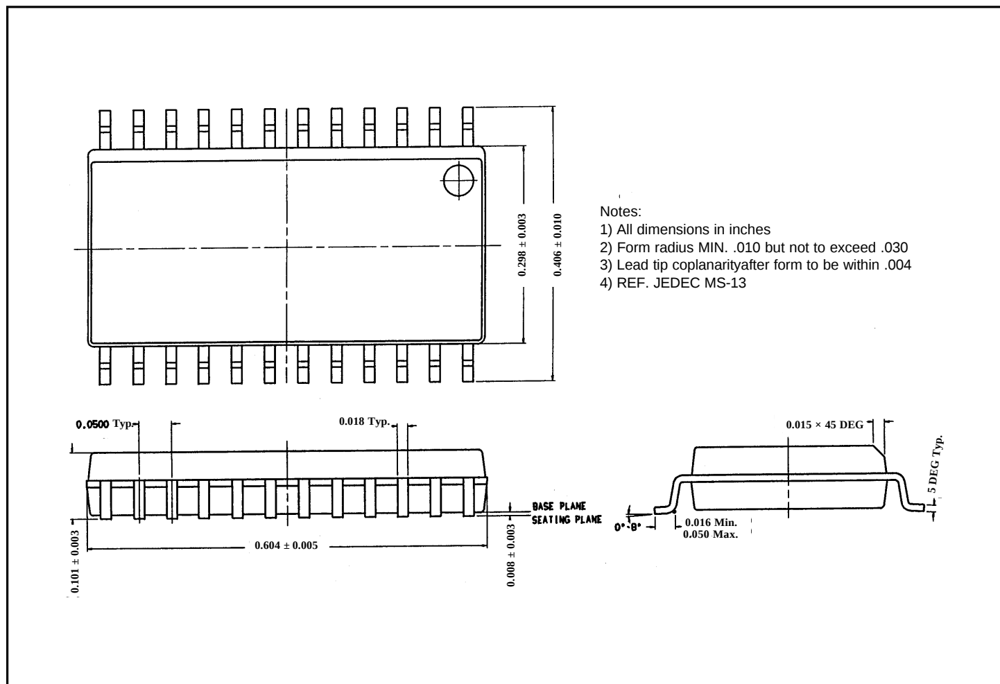
Figure 25. NW6003-XS 24 Pin SOIC Package Diagram
