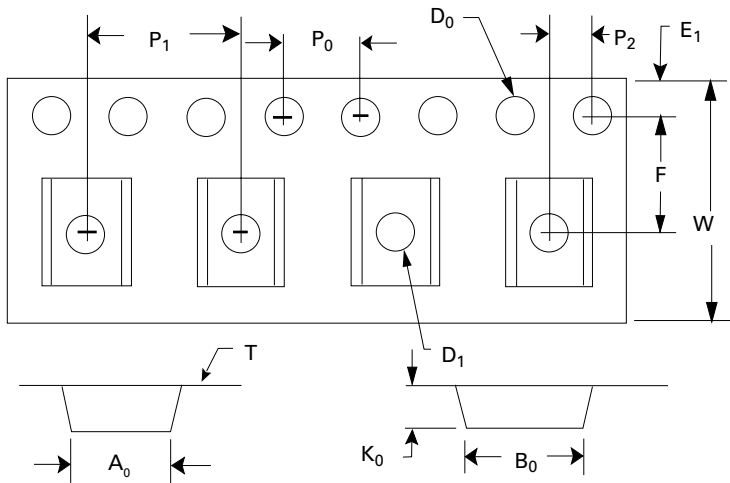
Tape Specifications
