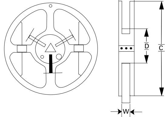
Reel Specifications
