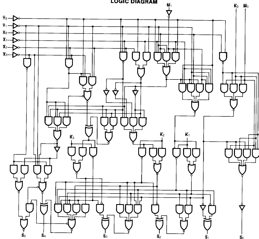
LOGIC DIAGRAM
