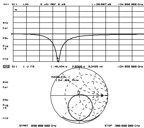
IF OUT Port Impedance ( P_{LO} = -15\text{dBm} , MIXER IN Port: 50ohm term.)
