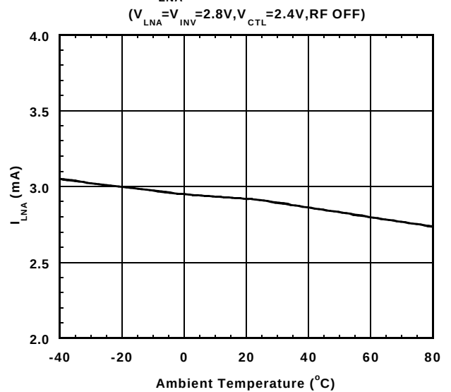
I_{LNA} vs. Temperature
