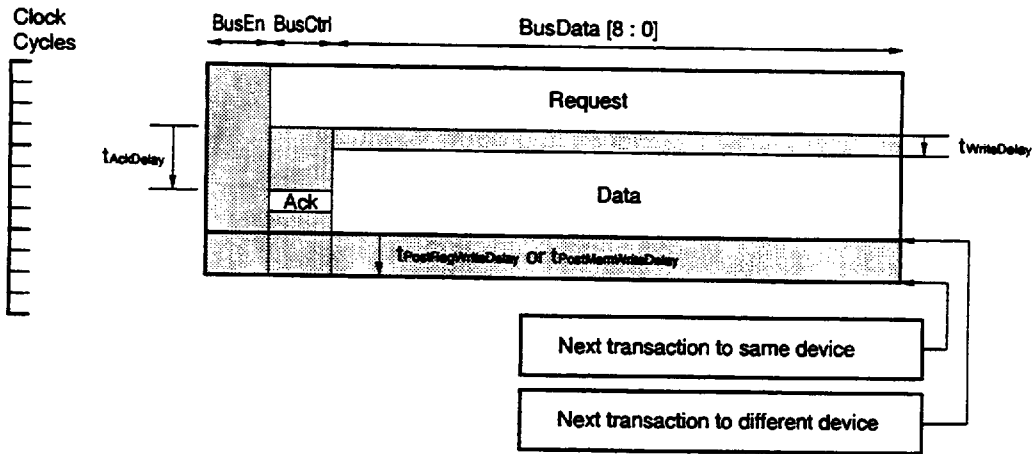
Figure 7-2. Write Transaction
