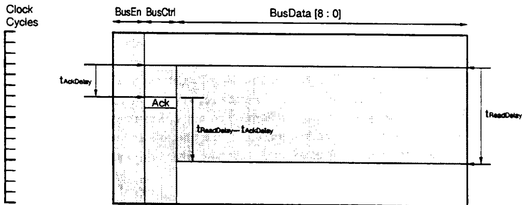
Figure 7-1. Read Transaction
