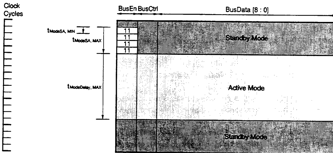
Figure 6-2. Basic ActiveMode/StandbyMode Transitions
