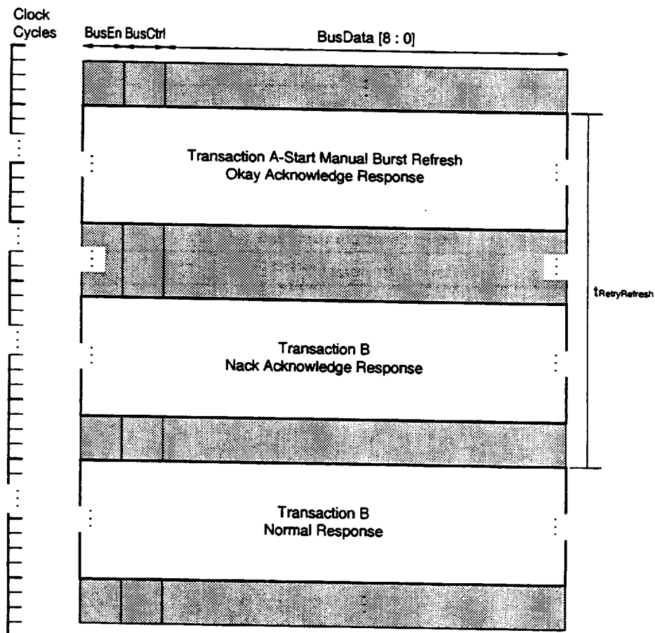
Figure 8-2. Transaction Holdoff Due to Burst Refresh
