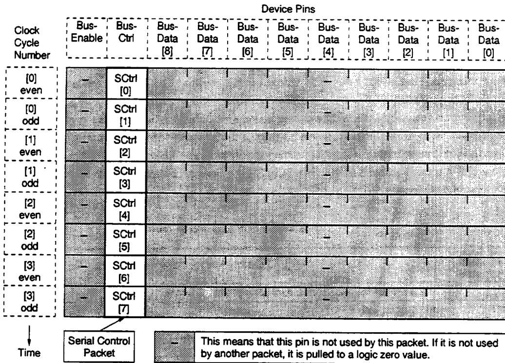
Figure 5-6. Serial Control Packet Format
