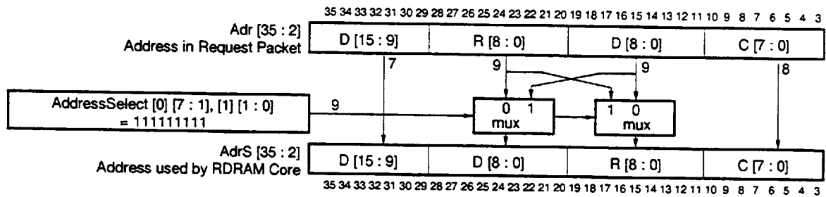
Figure 9-1. AddressMapping Hardware
