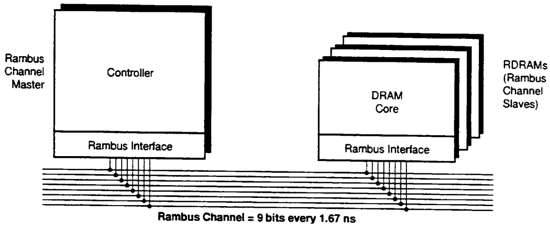
Figure 2-1. Logical Representation
