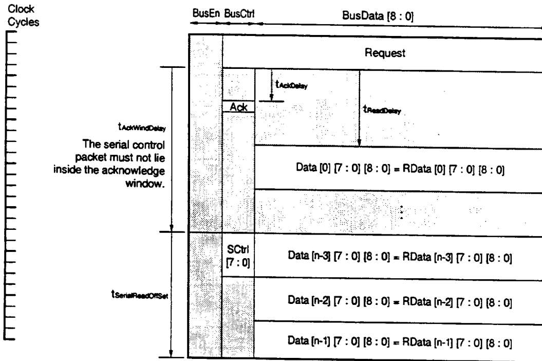
Figure 7-5. Read Transaction with Serial Control Packet
