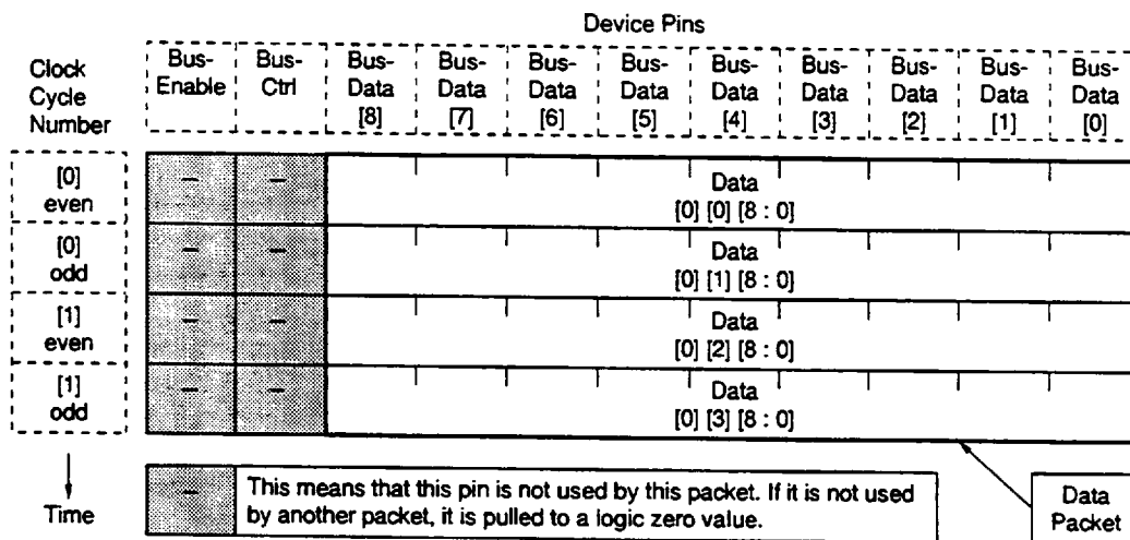
Figure 5-3. Data Packet Format (Register Space)
