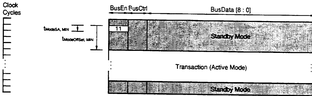
Figure 6-3. ActiveMode/StandbyMode Transition - Early Transaction
