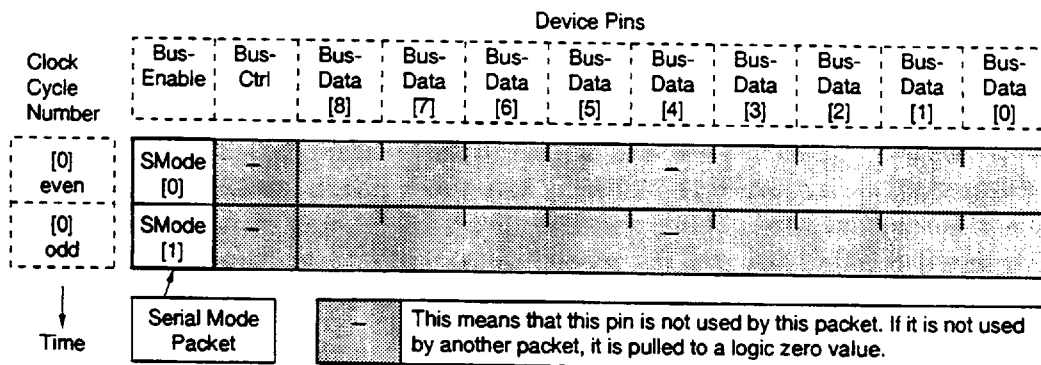
Figure 5-7. Serial Mode Packet Format
