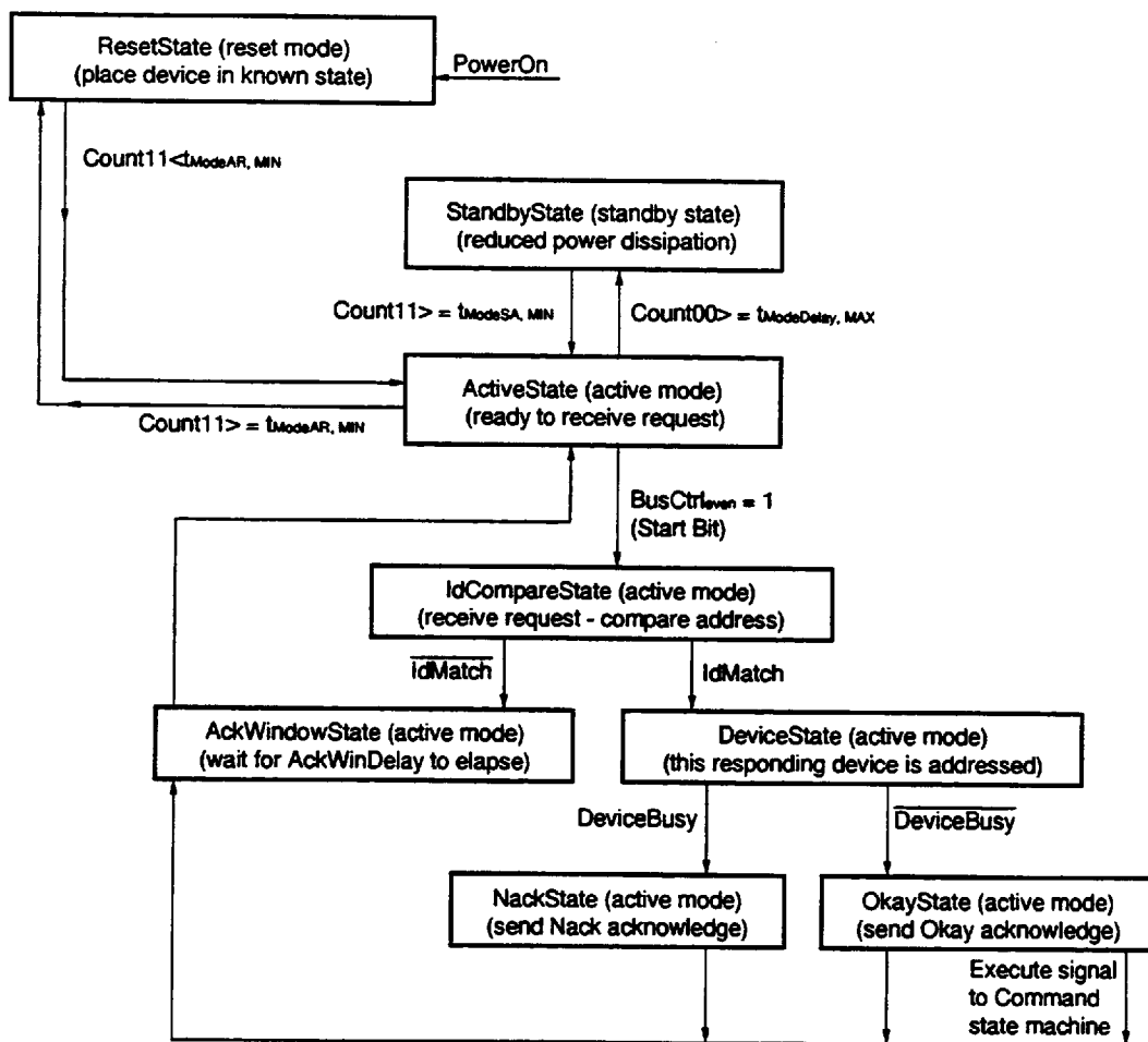
Figure 6-1. Frame State Machine - State Diagram
