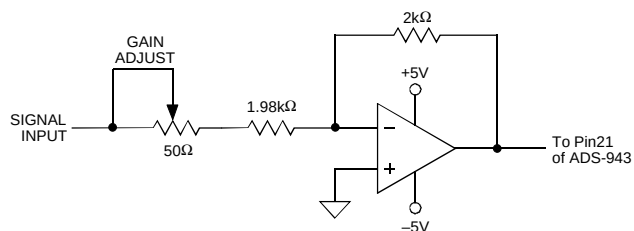
Figure 2. Optional ADS-943 Gain Adjust Calibration Circuit
