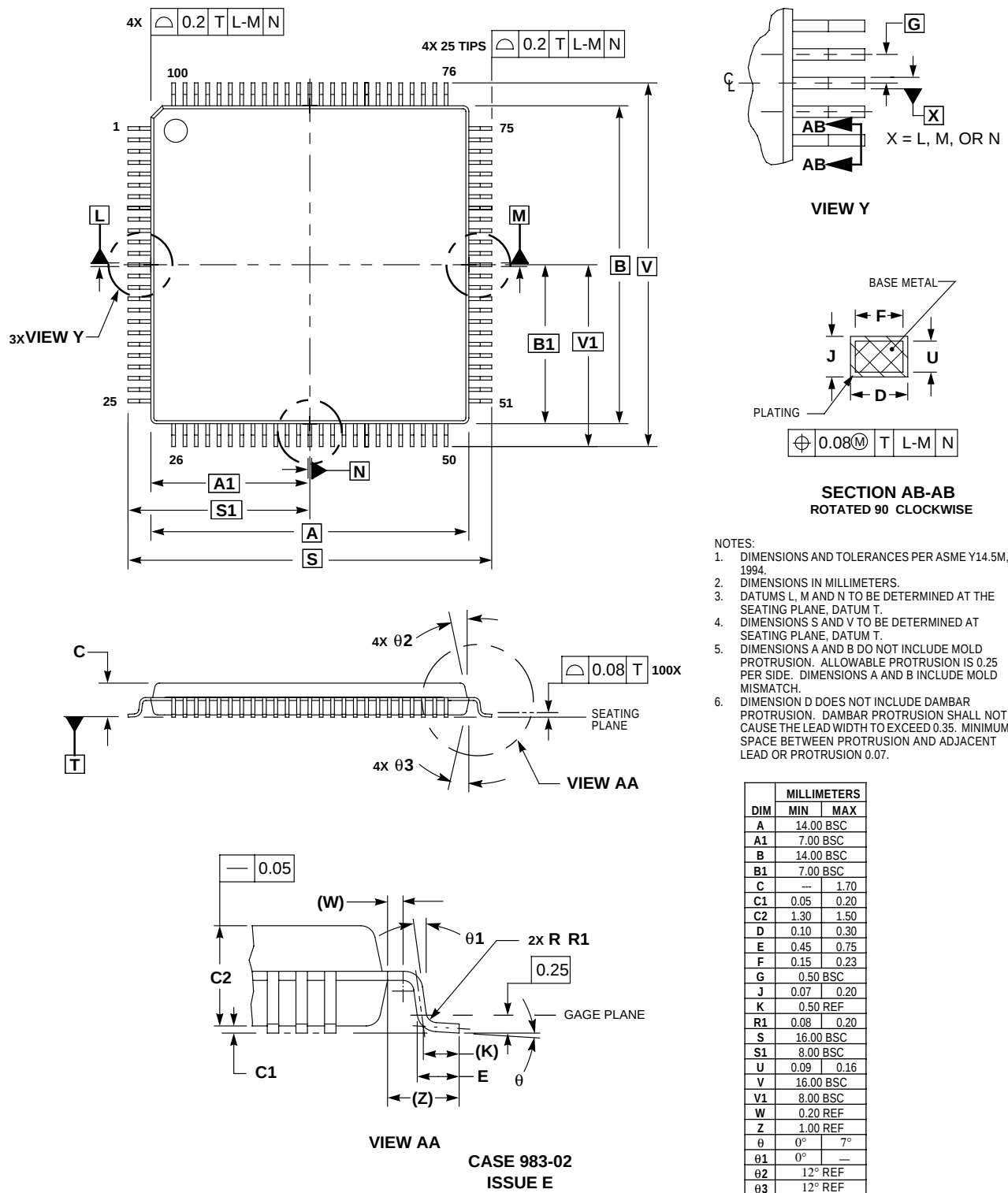
Figure 5-3. 100-Pin Thin Quad Flat Pack (TQFP) Mechanical Information
