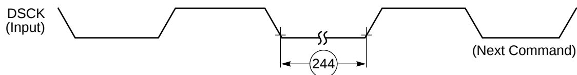
Figure 4-28. DSP56012 OnCE DSCK Next Command After Read Register Timing
