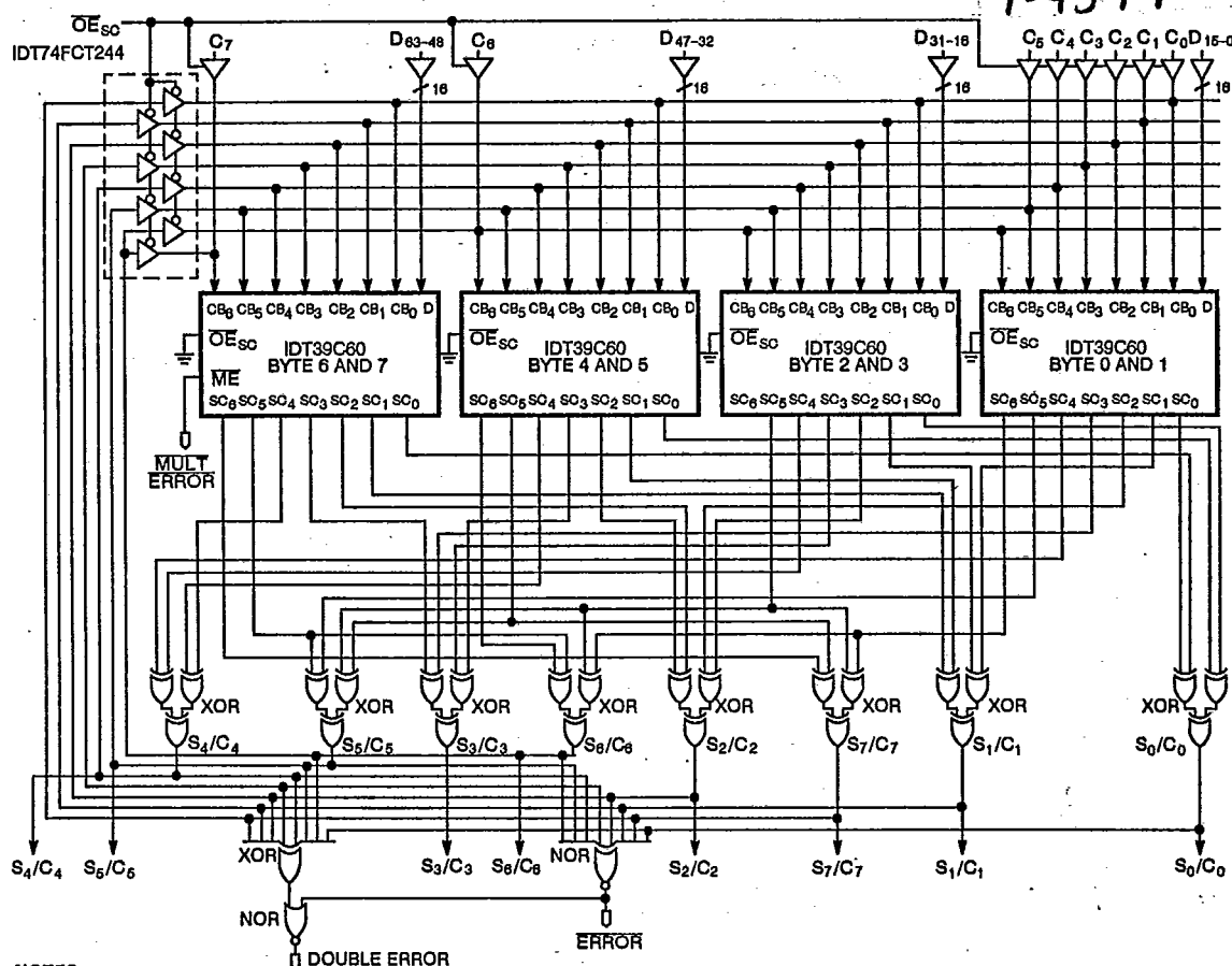
Figure 7. 64-Bit Configuration
