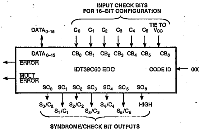
Figure 2. 16-Bit Configuration
