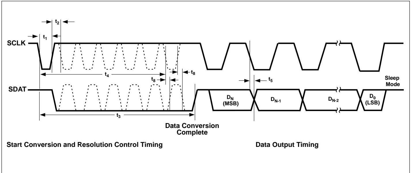
Figure 2. Conversion and Data Output Timing
