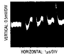
Figure 14. Poor Reference Settling Can Cause A/D Errors
