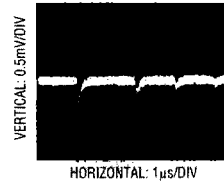
Figure 13. Adequate Reference Settling (LT1027)
