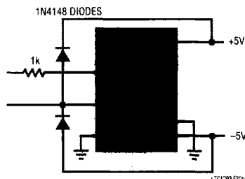
Figure 20b. Overvoltage Protection for Inputs
