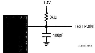
Load Circuit for t_{\text{enSSD}} and t_{\text{disSSD}}
