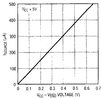
LTC1296 SS0 Source Current vs VCC - VSS0
