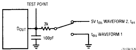
Load Circuit for t_{\text{dis}} and t_{\text{en}}
