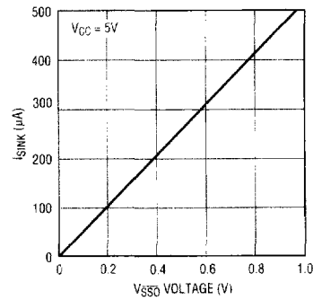
LTC1296 SS0 Sink Current vs VSS0
