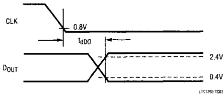
Voltage Waveform for D_{OUT} Delay Time, t_{dDQ}
