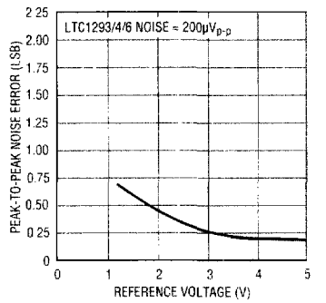
Noise Error vs Reference Voltage
