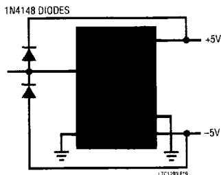
Figure 19. Overvoltage Protection for Inputs
