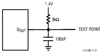
Load Circuit for t_{\text{DPO}} , t_r , and t_f
