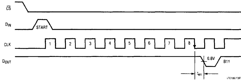
Voltage Waveforms for t_{en}
