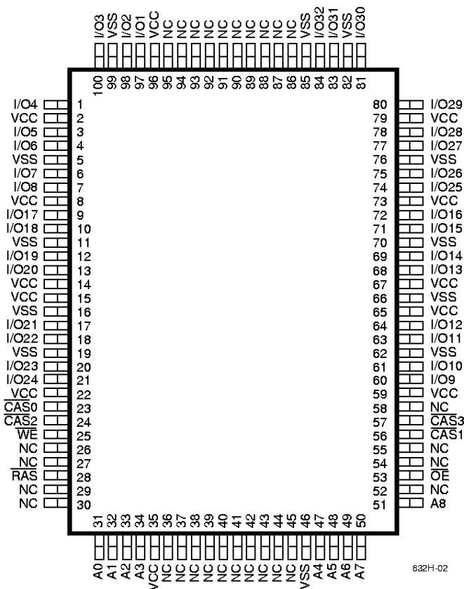
100-Pin PQFP/TQFP PIN CONFIGURATION Top View
