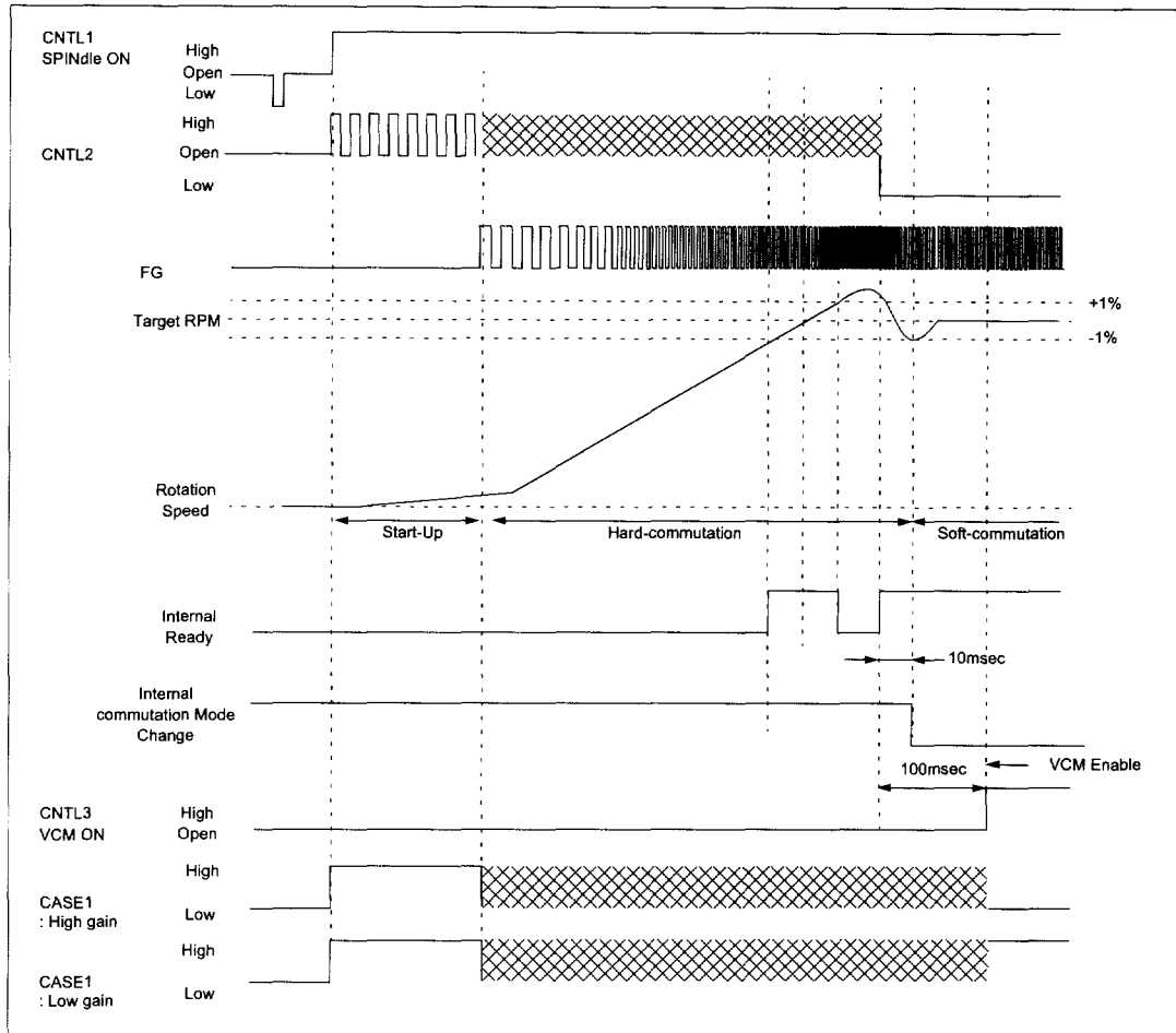
Figure 5. Motor start-up sequence
