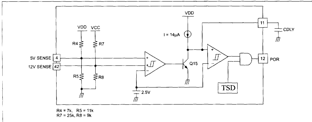
Figure 12. Power on reset block schematic
