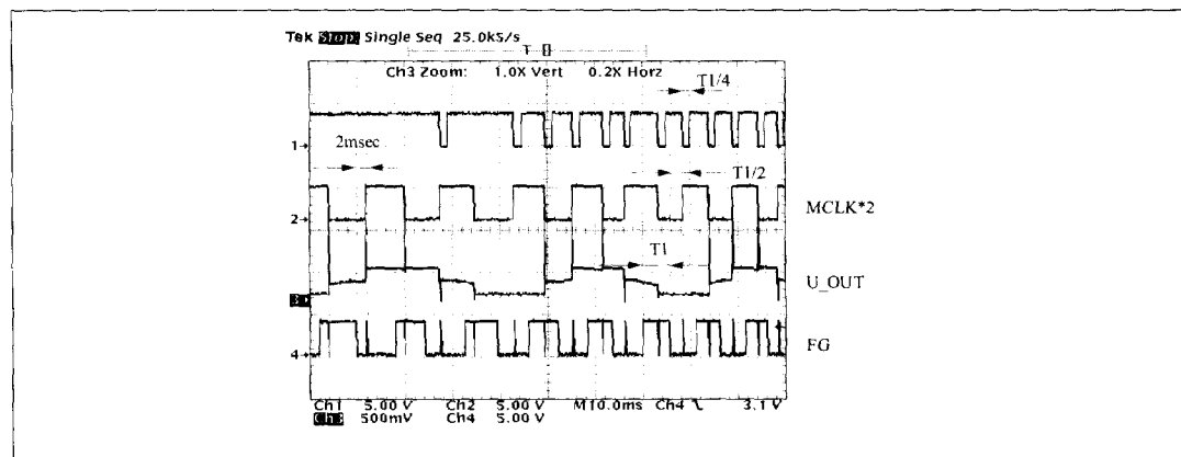
Figure 17. Acceleration mode 2
