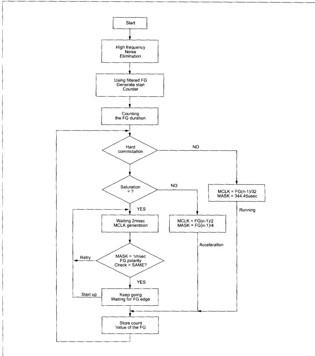
Figure 8. MCLK generation flow chart
