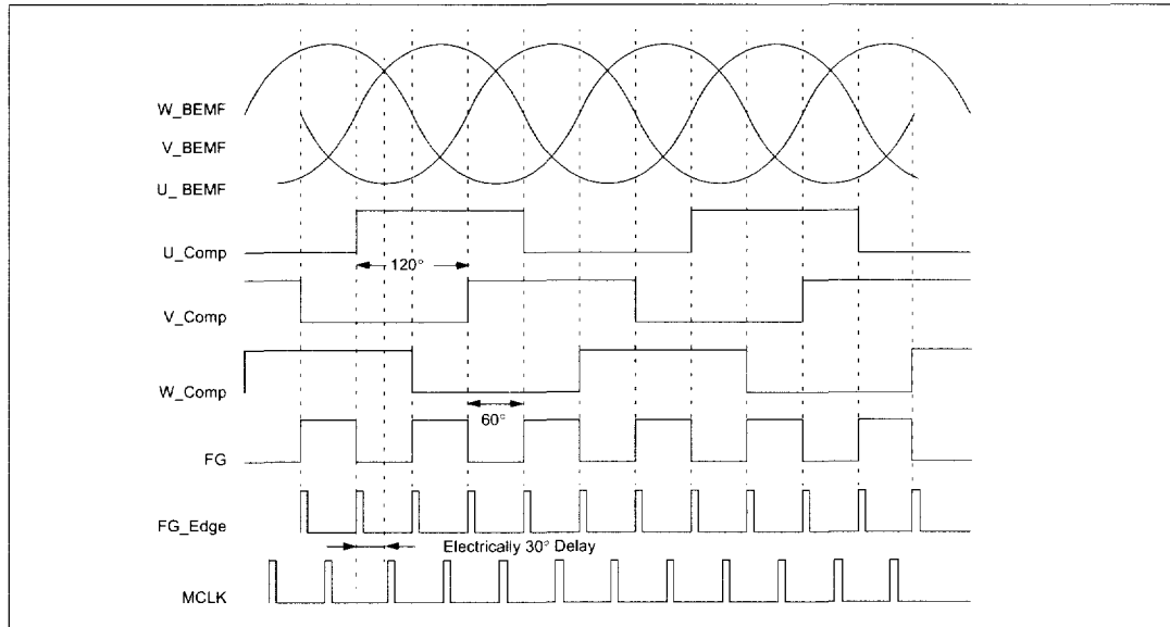
Figure 1. BEMF, FG, and MCLK in the acceleration mode
