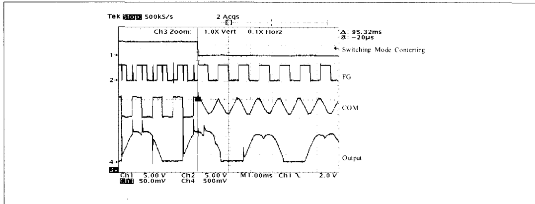
Figure 19. commutation mode converting
