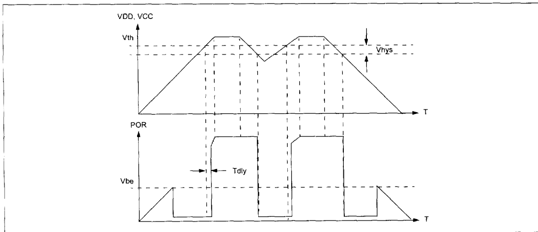
Figure 13. Power on reset function
