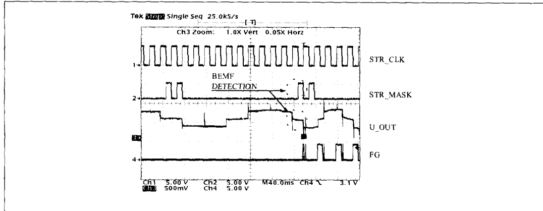
Figure 15. Start-up mode
