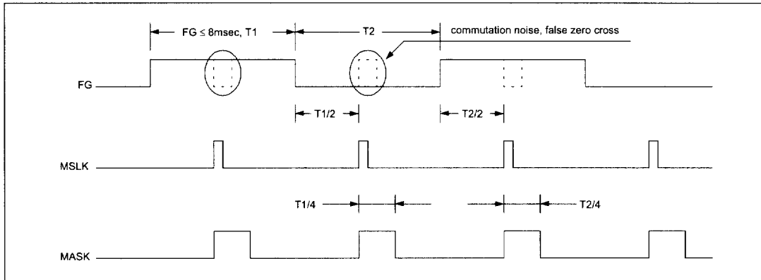
Figure 3. MCLK vs MASK in the acceleration mode
