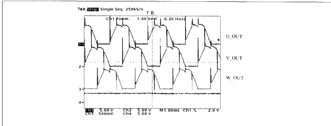
Figure 18. Output in hard-commutation mode
