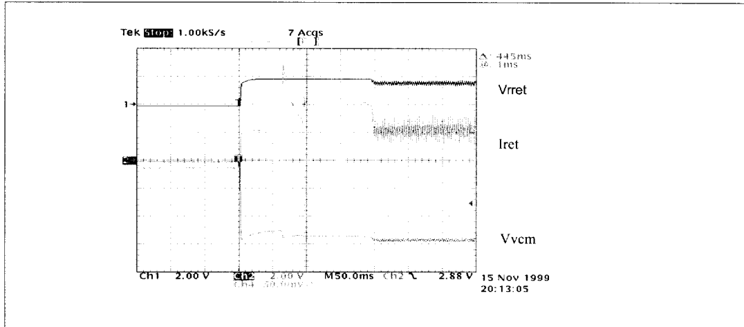
Figure 22. Retract &amp; break at power off
