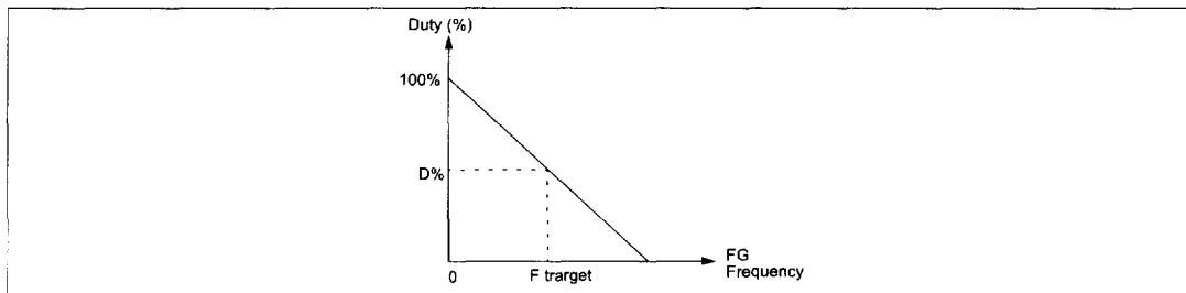
Figure 6. FG vs PWMSD duty variation
