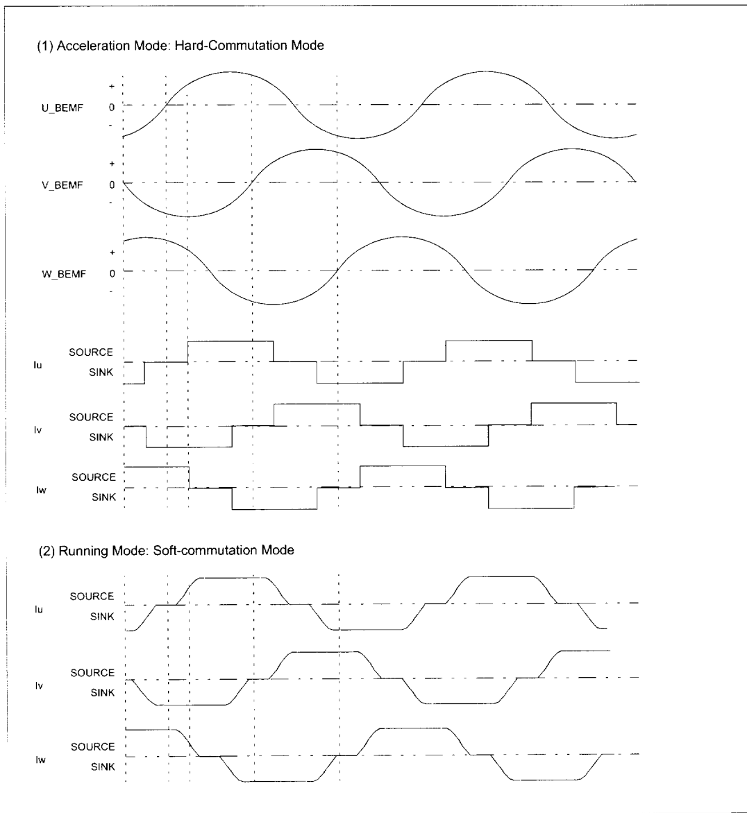
Figure 7. Acceleration and running the spindle motor
