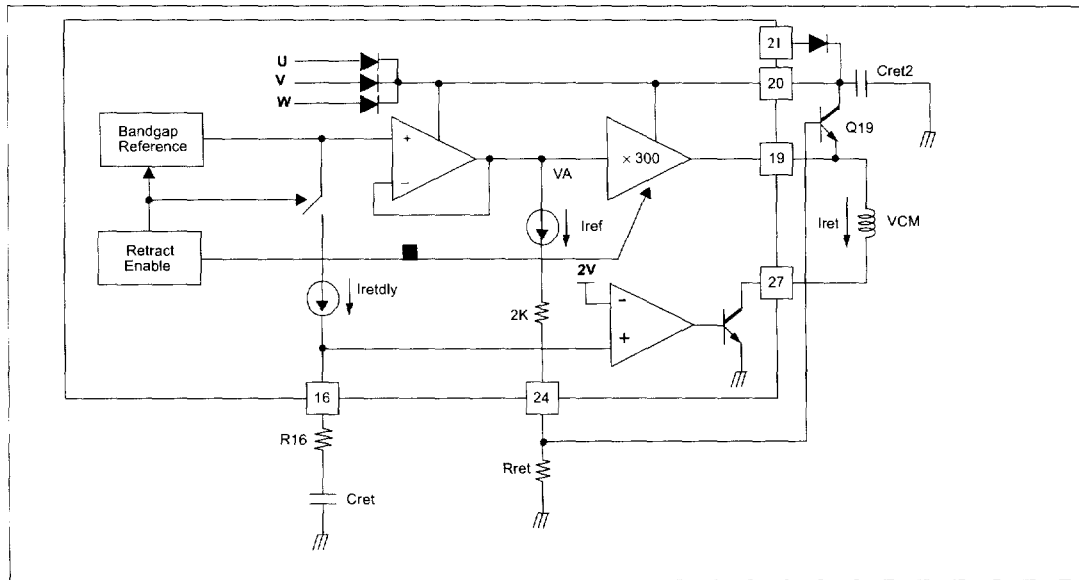
Figure 11. Retract block schematic
