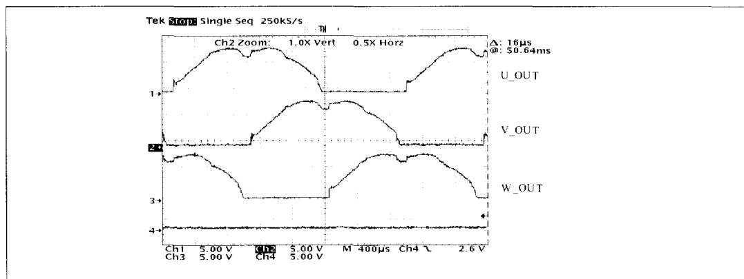
Figure 20. Soft-commutation mode
