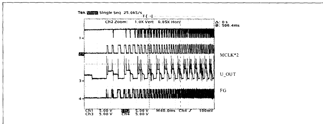
Figure 16. Acceleration mode 1
