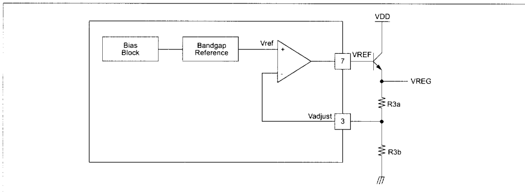
Figure 14. low drop regulator schematic
