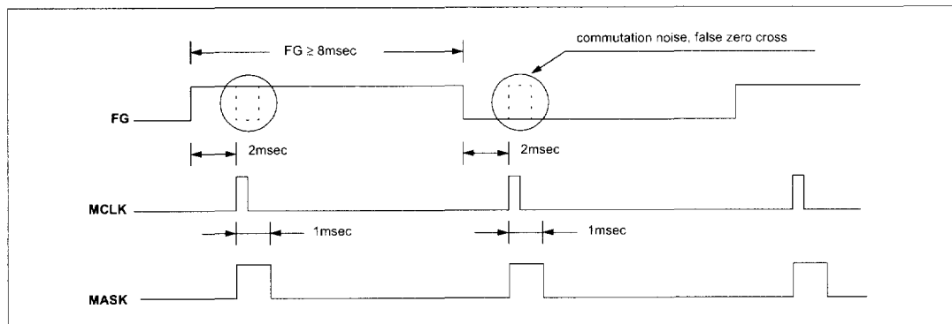
Figure 2. MCLK vs MASK in the start-up mode
