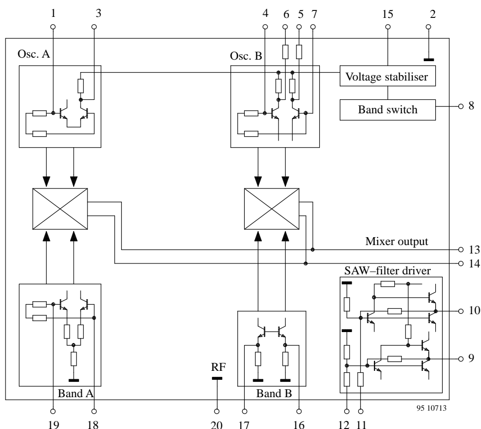
Figure 1. Block diagram
