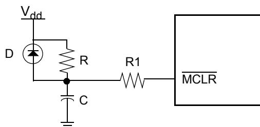
Figure 12-5. External Power-On Reset Circuit (For Slow V_{\text{dd}} Power-up)
