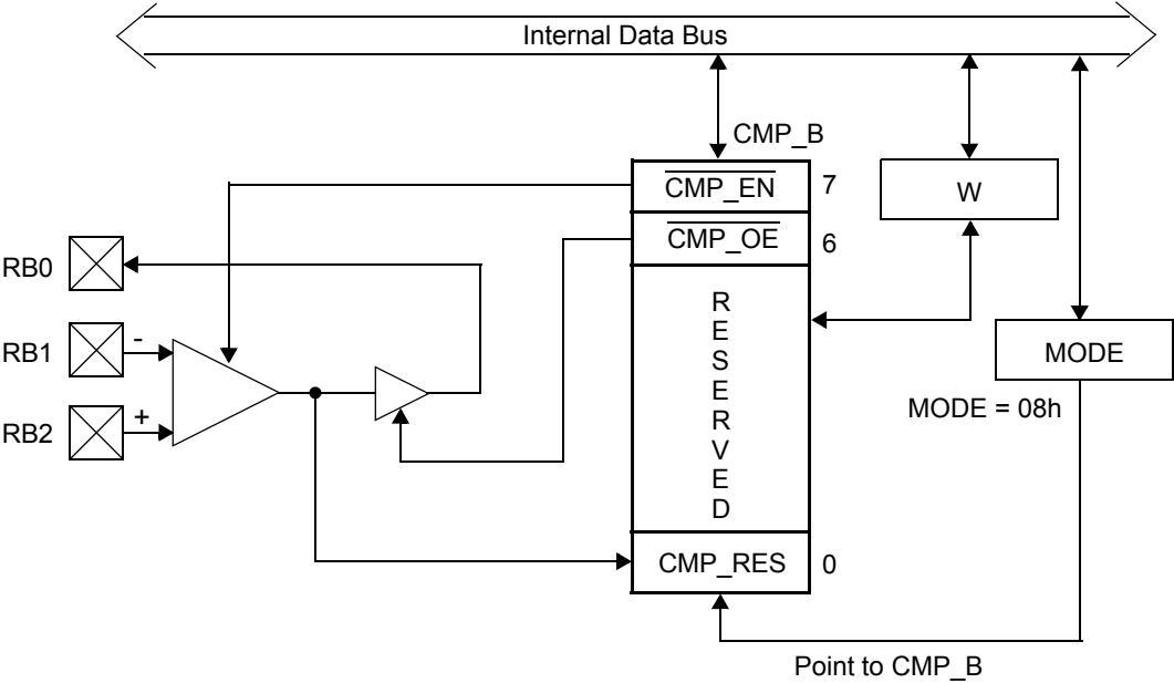
Figure 11-1. Comparator Block Diagram
