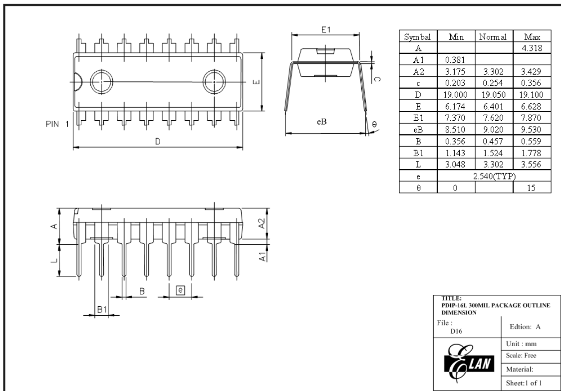
Figure C-1 EM78F562N/F662N 16-pin PDIP Package Type
