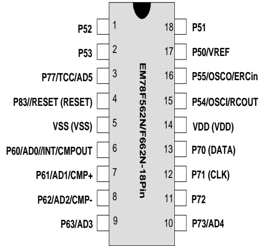
Figure 3-2 EM78F562N/F662ND18/SO18
