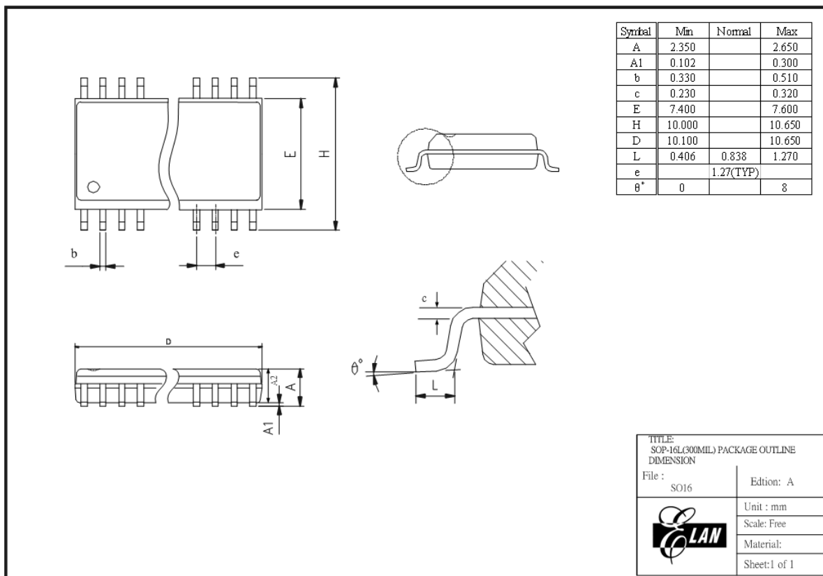
Figure C-2 EM78F562N/F662N 16-pin SOP Package Type
