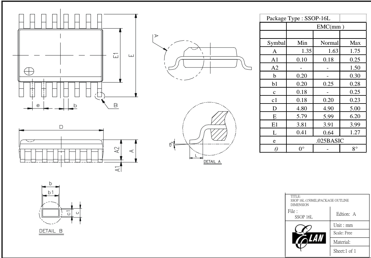
Figure C-4 EM78F662N 16-pin SSOP Package Type
