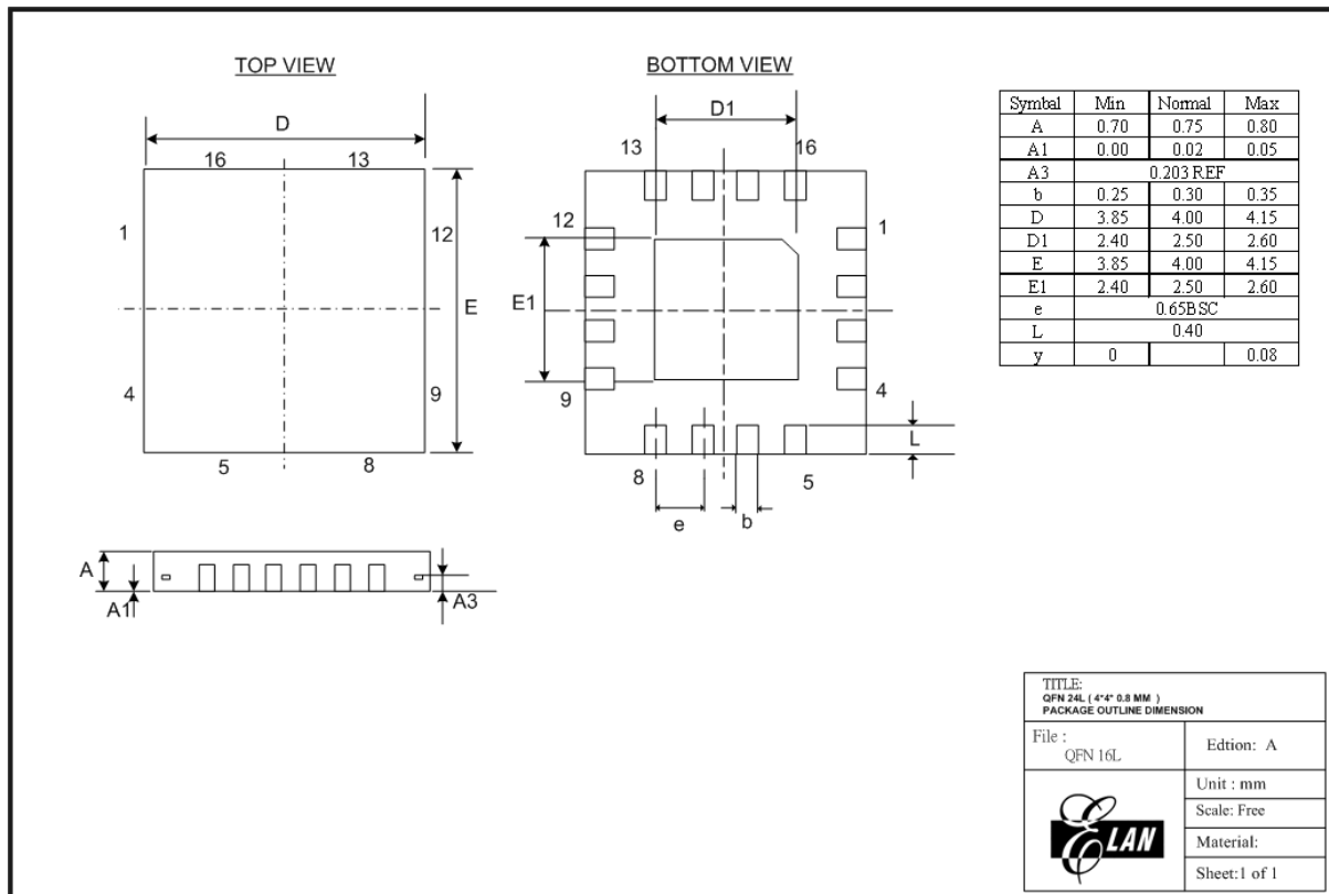
Figure C-3 EM78F662N 16-pin QFN Package Type
