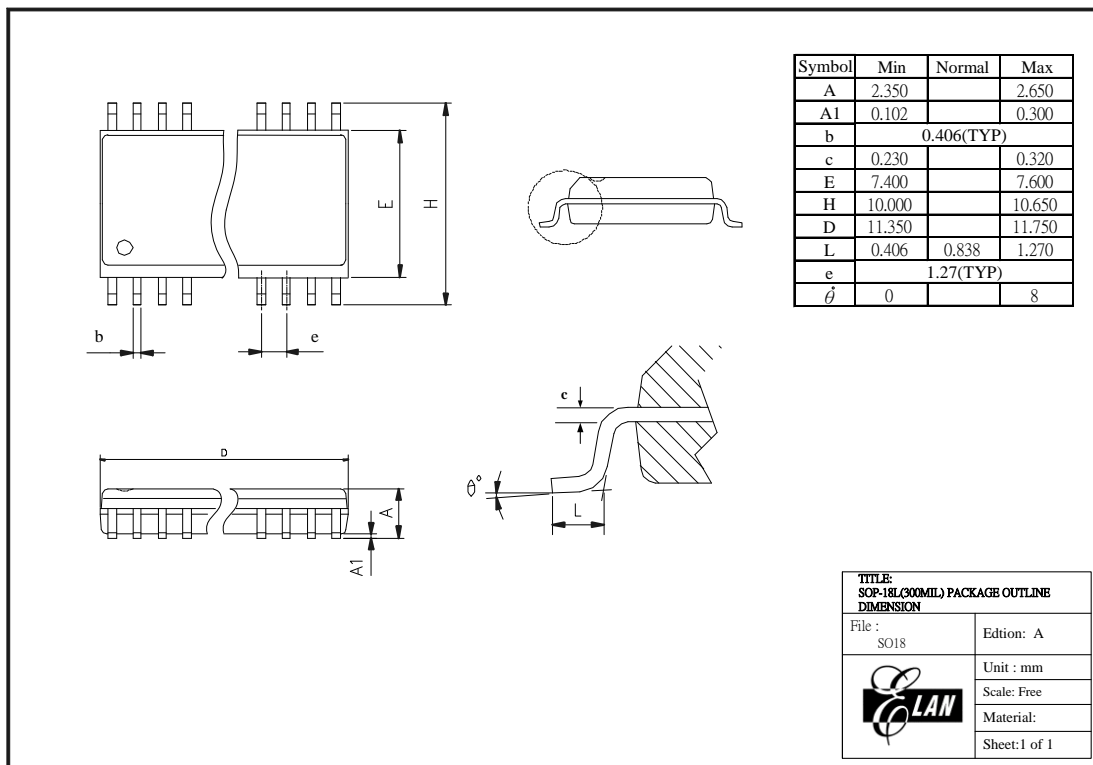
Figure C-6 EM78F562N/F6622N 18-pin SOP Package Typ
