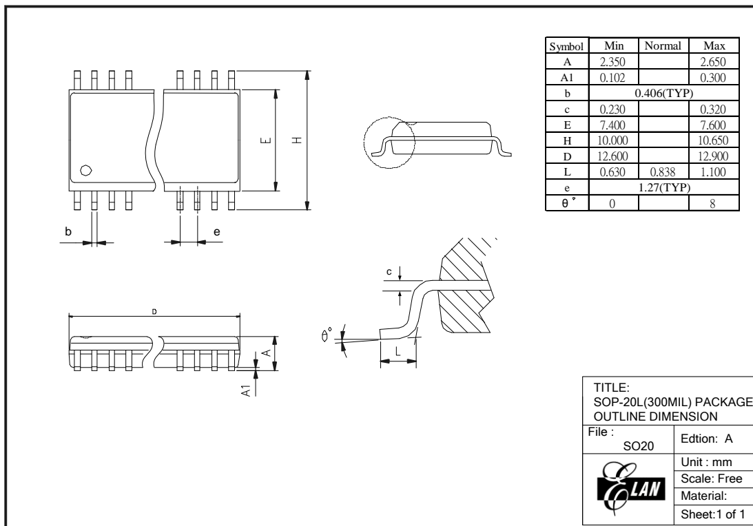
Figure C-8 EM78F562N/F662N 20-pin SOP Package Typ
