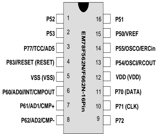
Figure 3-1 EM78F562N/F662ND16/SO16
