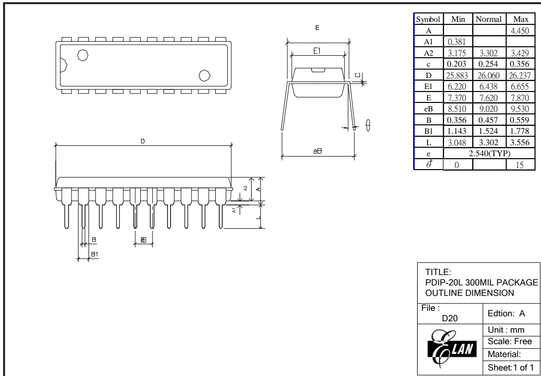
Figure C-7 EM78F562N/F662N 20-pin PDIP Package Type
