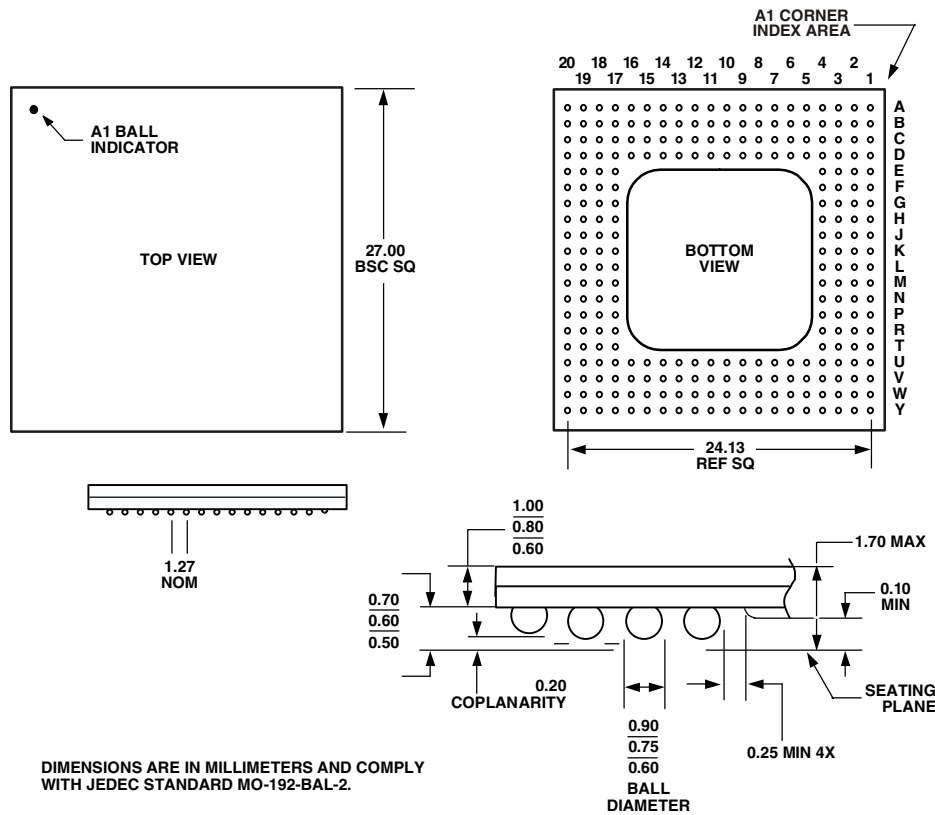
Figure 42. 256-Ball SBGA, Thermally Enhanced (BP-256)
