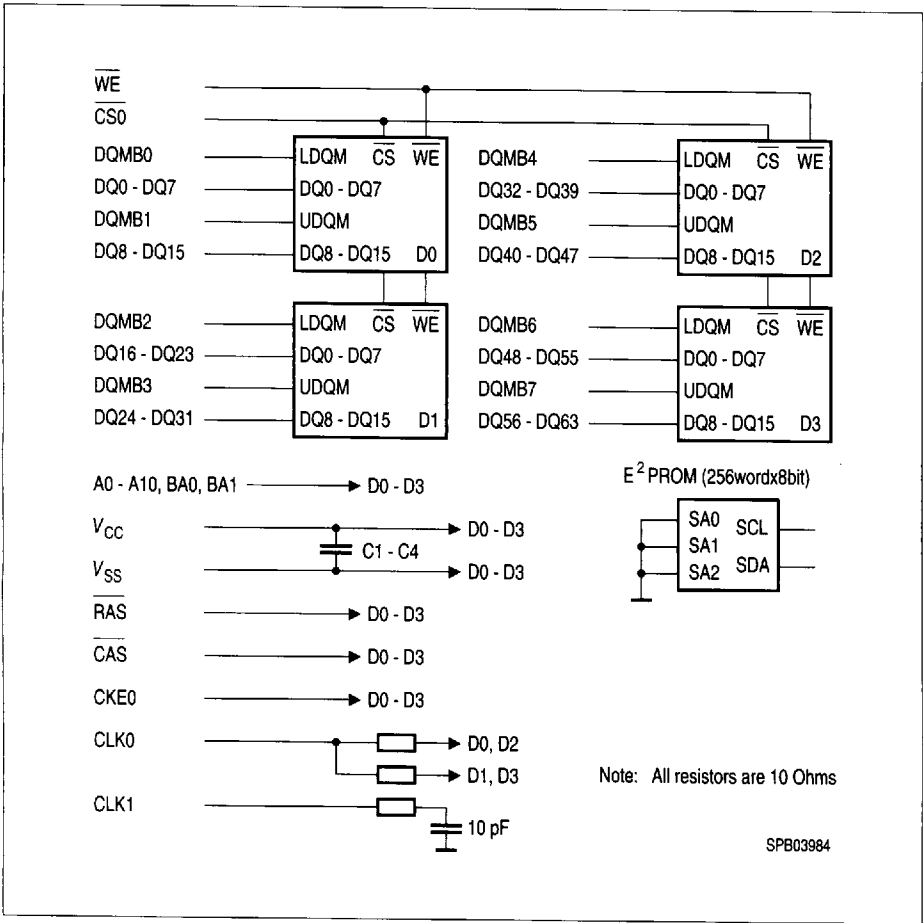
Block Diagram for 4M x 64 SDRAM - DIMM Module
