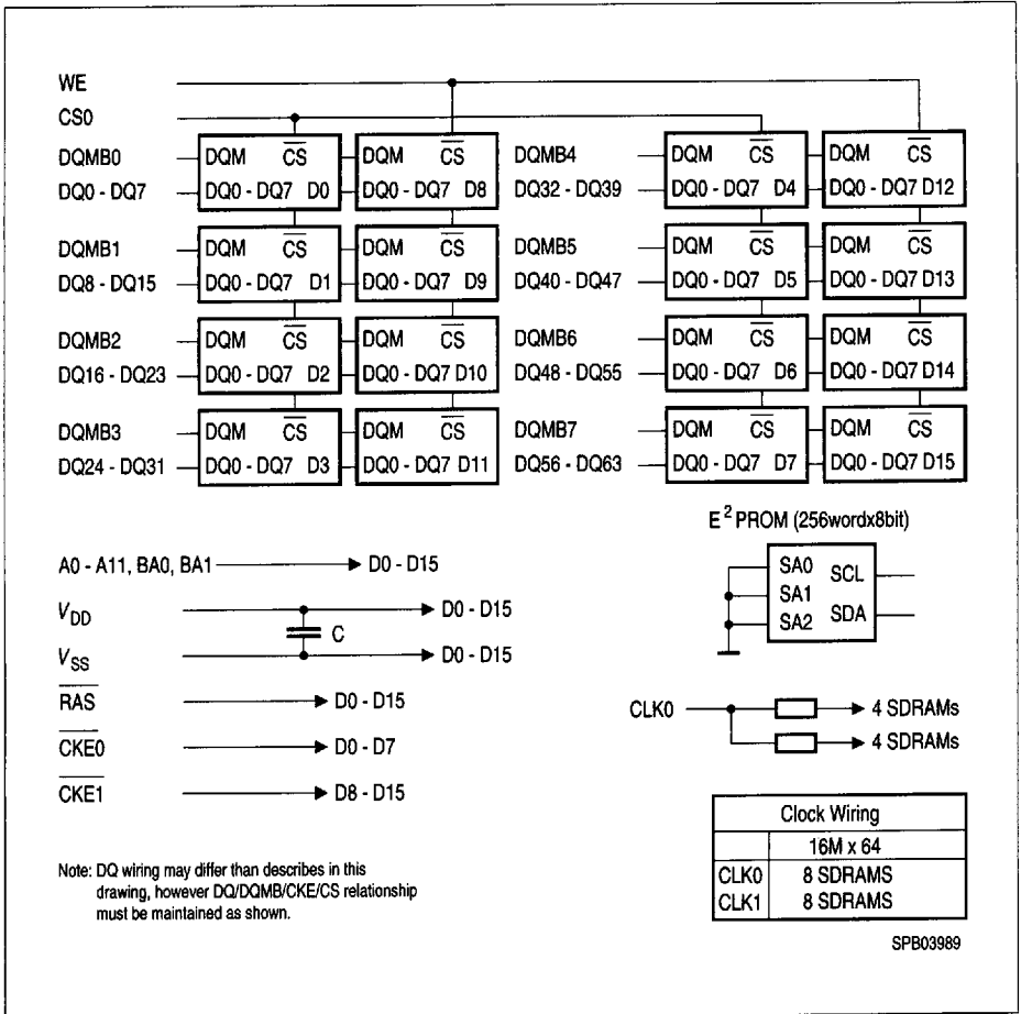
Block Diagram for Two Bank 16M x 64 SDRAM DIMM - Module (8M x 8 based)
