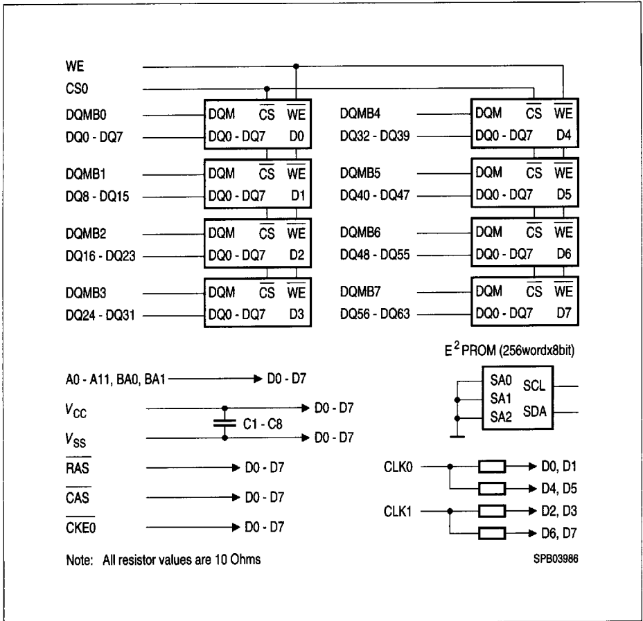
Block Diagram for 8M x 64 SDRAM DIMM - Module
