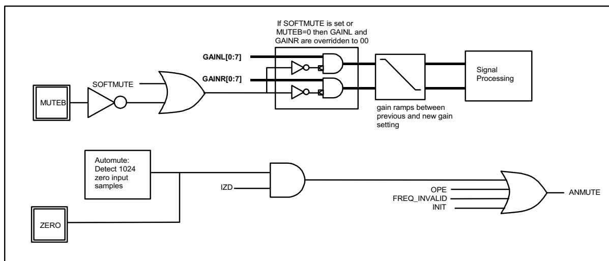
Figure 7 Mute Modes
