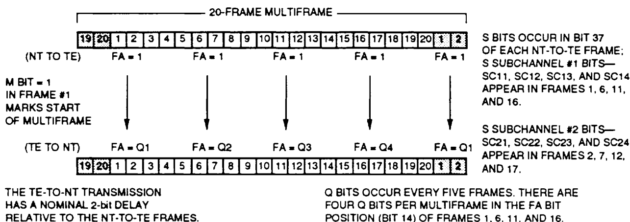
Figure 8. 20-Frame Multiframe
