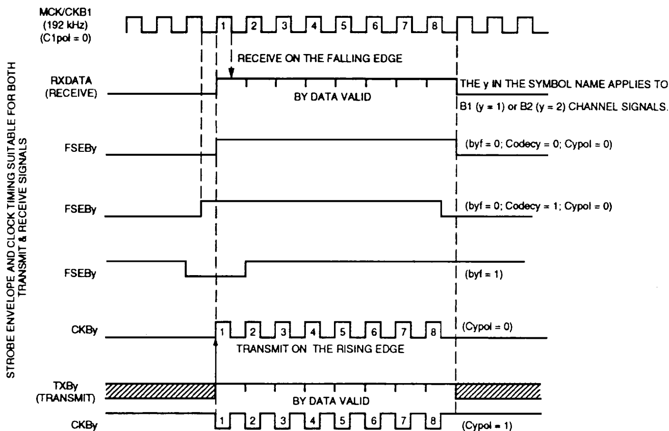
Figure 20. Bit Alignment Timing, with Programmable Options, on the System Interface
