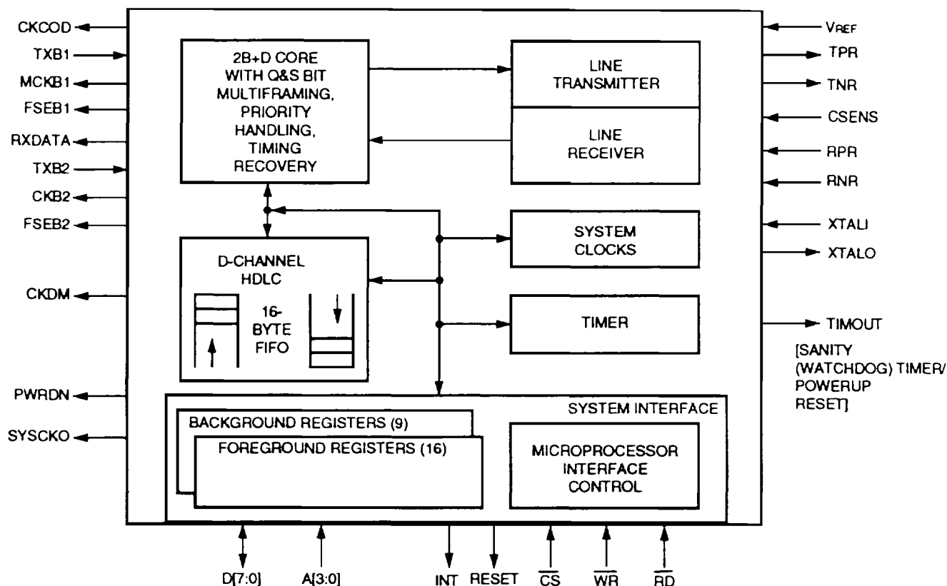
Figure 1. Block Diagram
