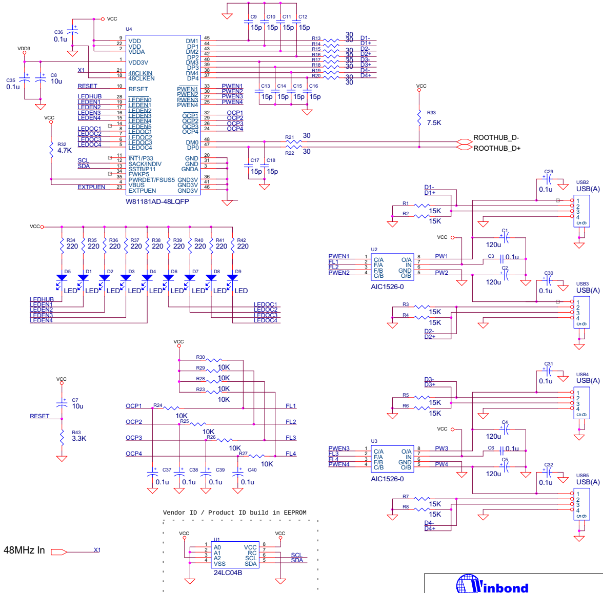
W81181AD USB Hub Reference Schematic (48MHz for Mother Board)
