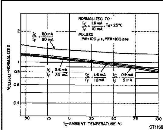
Fig. 3. V_{CE(sat)} vs. Temperature
