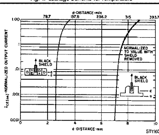
Fig. 6. Output Current vs. Shield Distance
