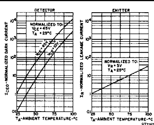
Fig. 4. Leakage Currents vs. Temperature
