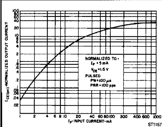
Fig. 1. Output Current vs. Input Current
