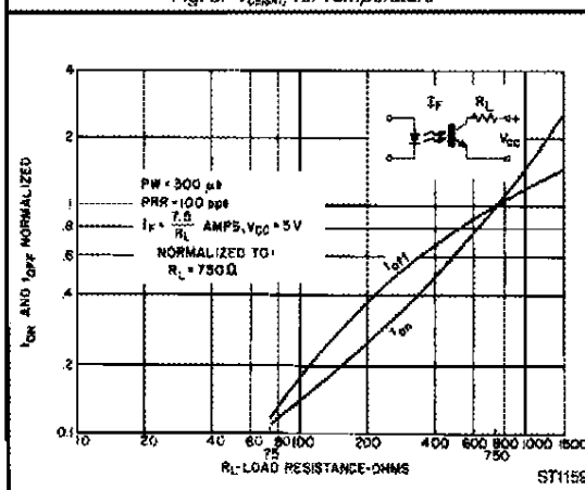
Fig. 5. Switching Speed vs. R_L
