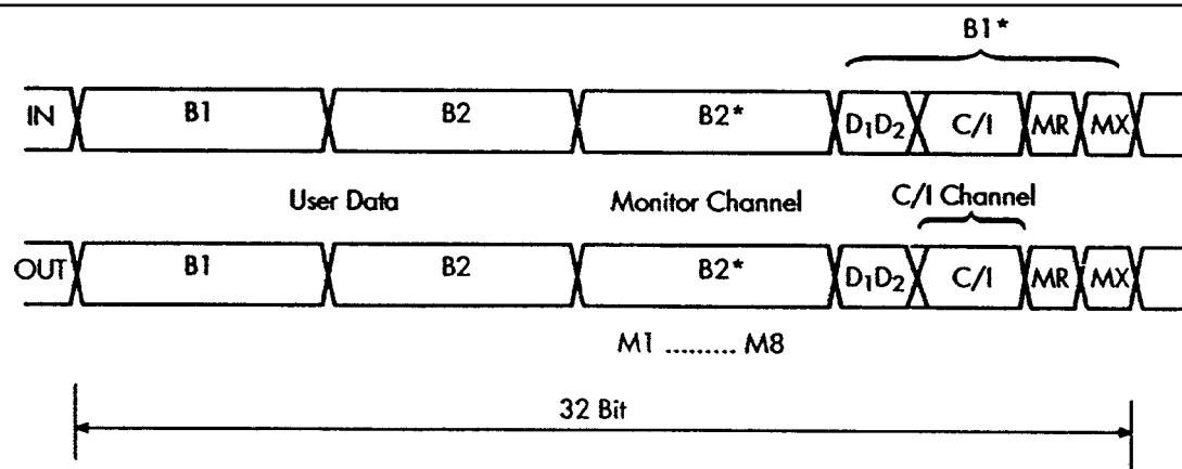
Fig. 4.2 : Frame Structure GCI
