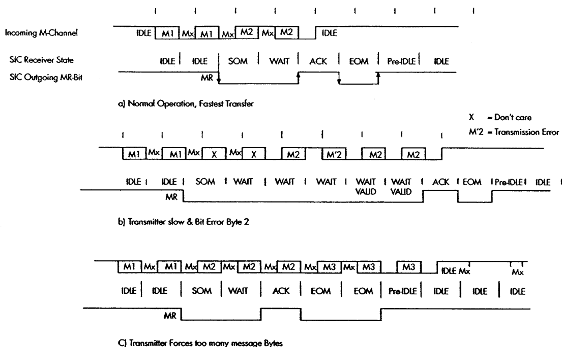
Fig. 6.13 : Examples of Received M-Channel Messages
