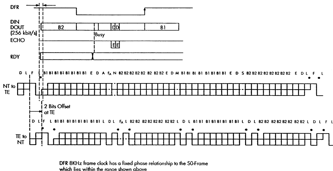
Fig. 5.5 : GCI S-bus Phase Relation TE Mode, RDY & ECHO pin
