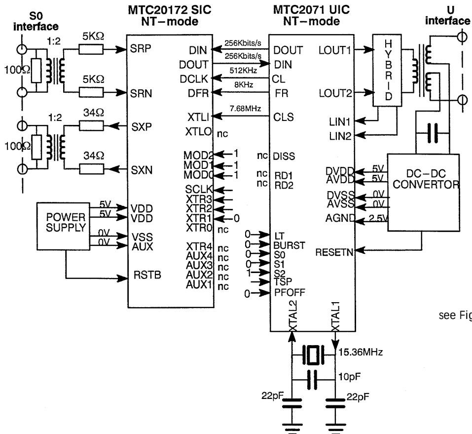
Fig. 13.1 : MTC-20172 SIC in NT mode with MTC2071 UIC
