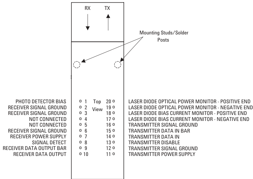
Figure 5. Pin Out Diagram (Top View)
