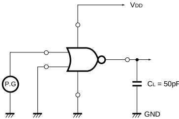
Fig.2 Switching characteristics
