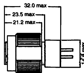
MC406E-* -09-02 ** Plug
