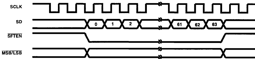
FIGURE 2A. FREQUENCY LOADING ENABLED BY SFTEN
