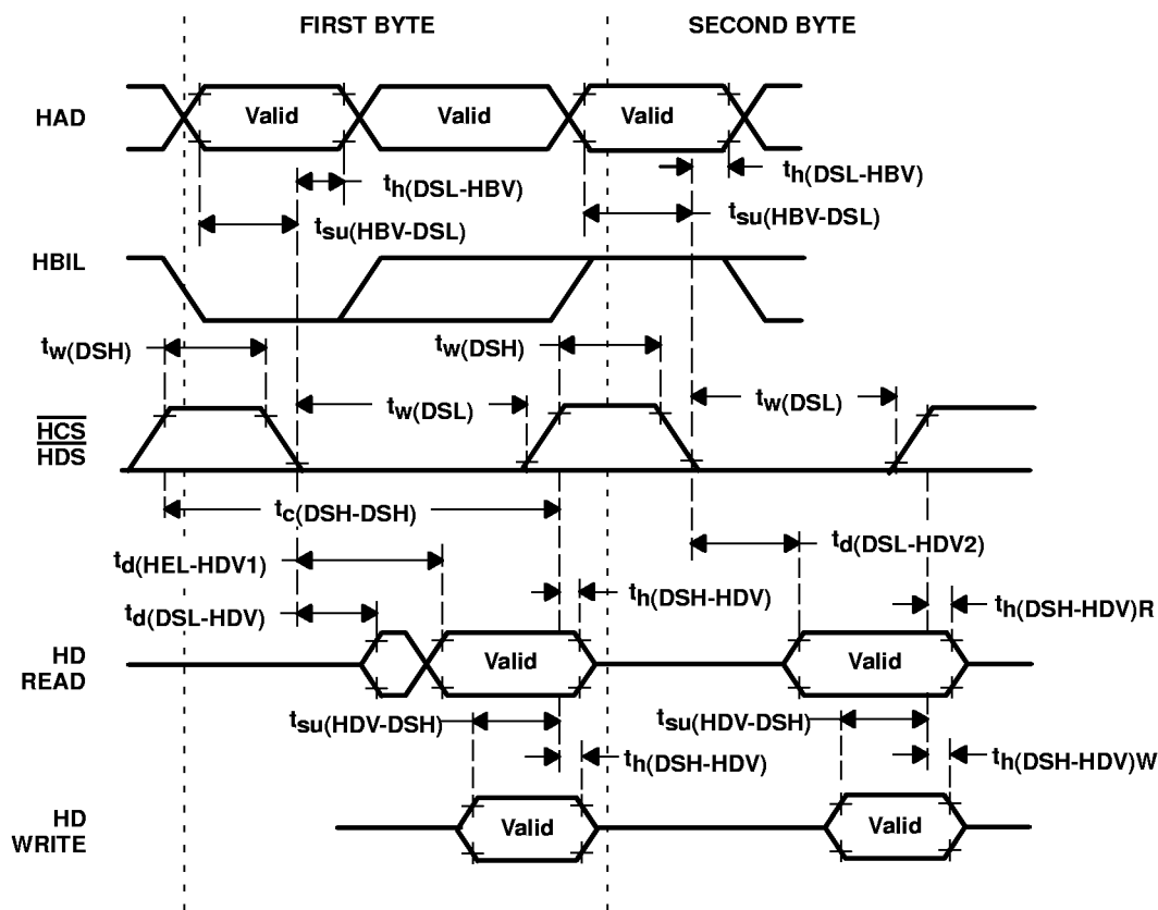
Figure 40. Read/Write Access Timings Without HRDY or HAS
