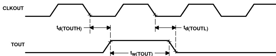
Figure 31. TOUT Timing
