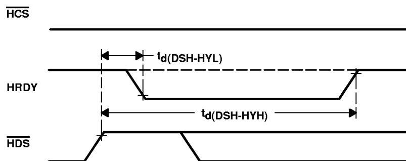
Figure 43. HRDY Signal When \overline{HCS} is Always Low
