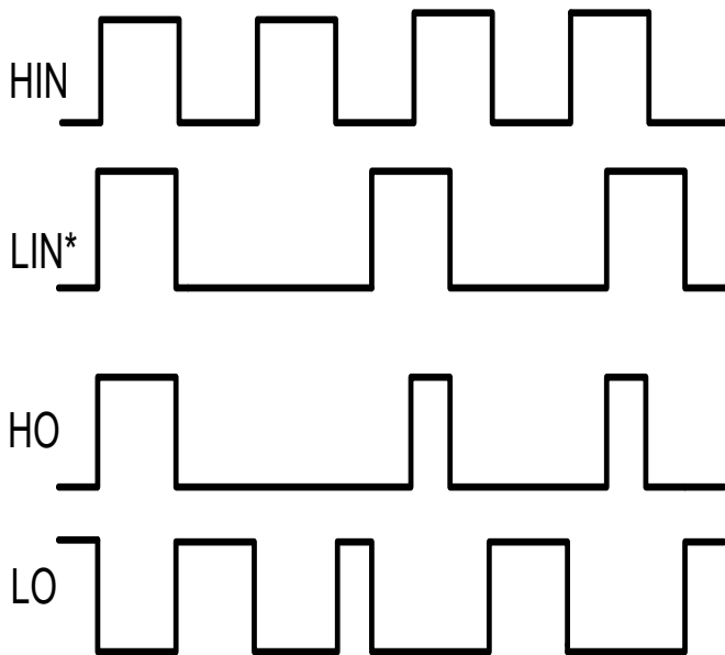
Figure 1. Input / Output Logic Diagram
