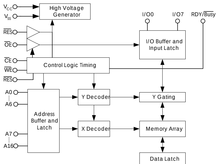
Logic Diagram
