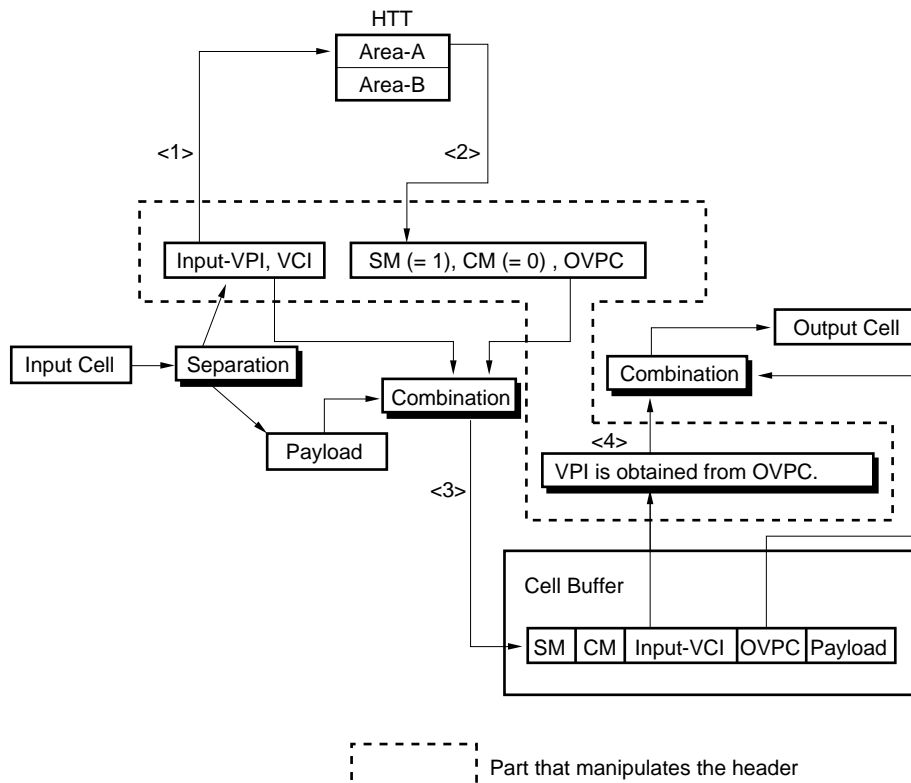
Figure 3-31. Flow of Header Translation in VPC and Single Cast Modes
