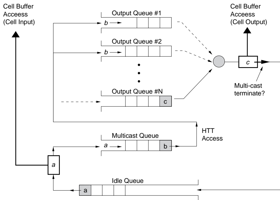
Figure 3-34. Queuing of Cell Address (Multi-Cast)
