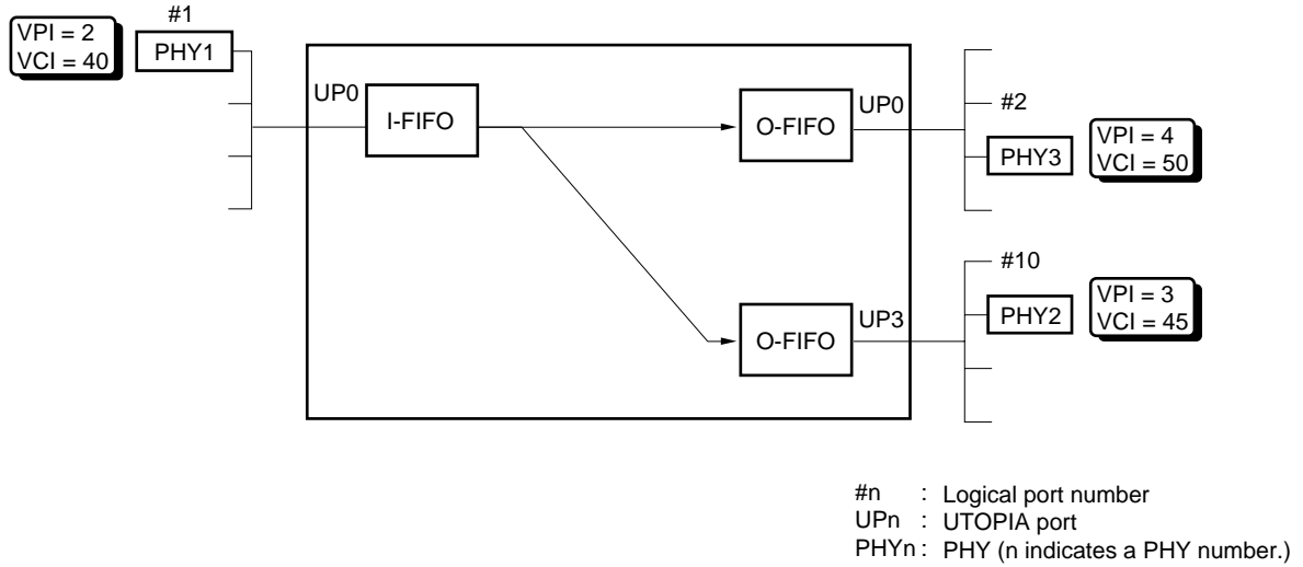
Figure 3-21. Example of Multi-Cast
