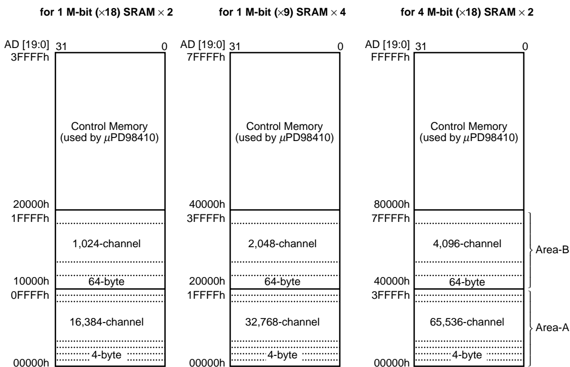
Figure 3-17. HTT & Control Memory Map
