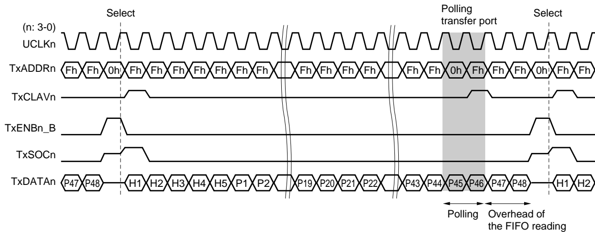
Figure 3-45. Polling Timing (b)
