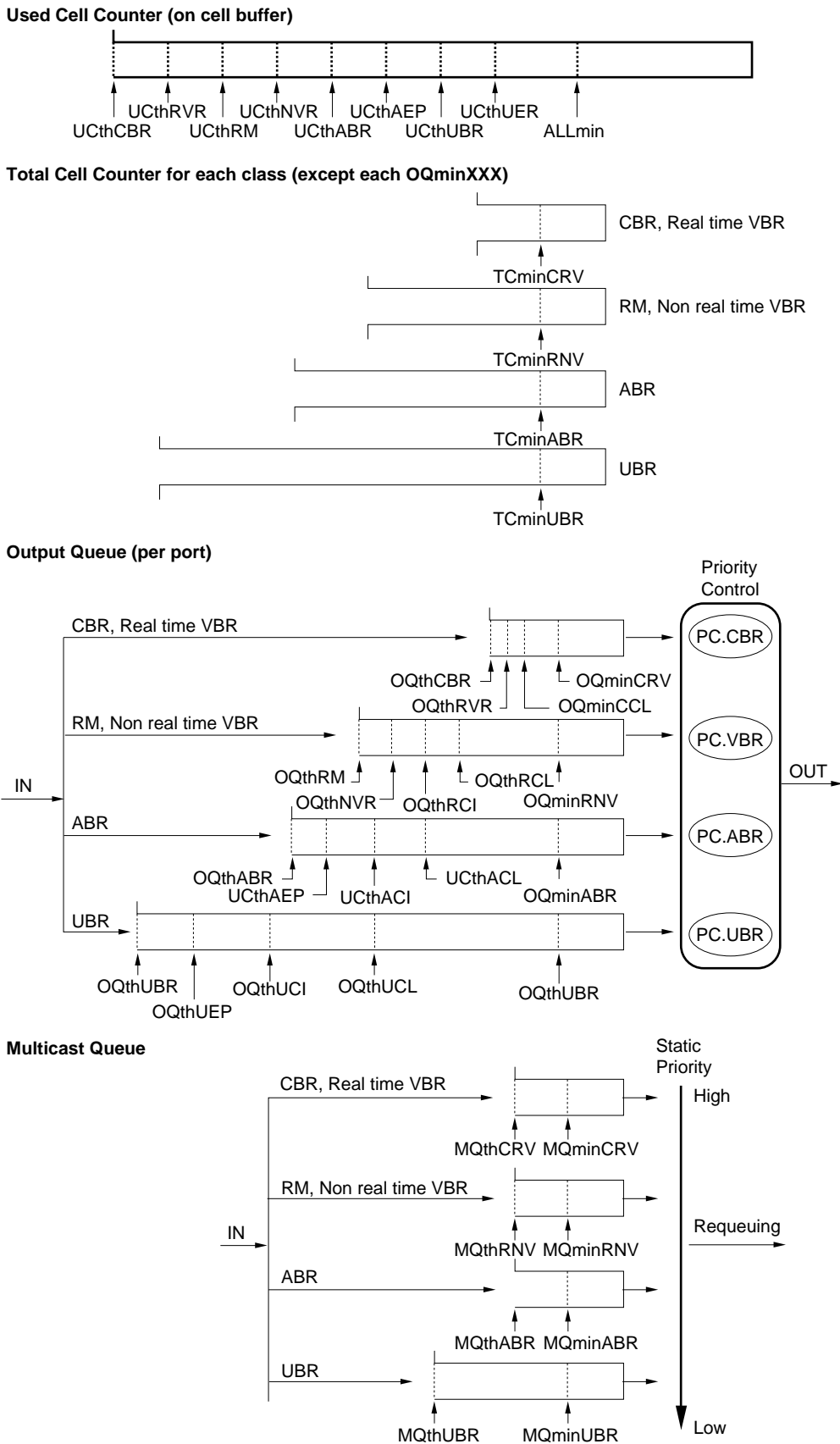
Figure 3-35. Queues and Counters by Service Class
