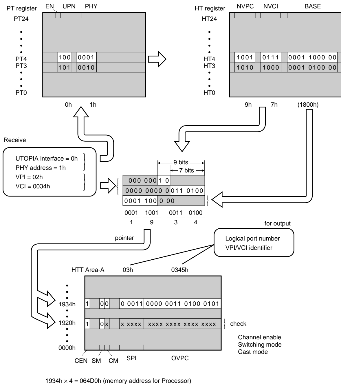
Figure 7-2. Header Translation Flow (reception side)
