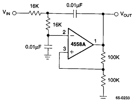
Figure 23. DC Coupled 1kHz Low-Pass Active Filter
