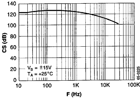
Figure 15. Channel Separation vs. Frequency
