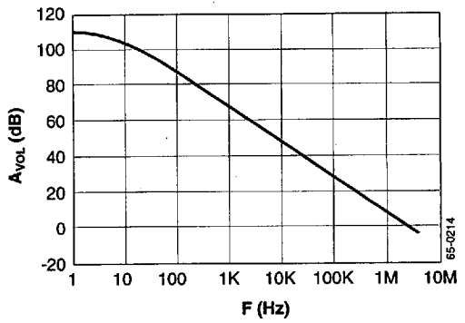
Figure 4. Open Loop Voltage Gain vs. Frequency
