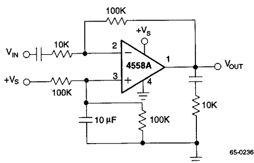
Figure 25. AC Coupled Inverting Amplifier
