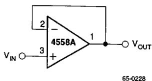
Figure 18. Voltage Follower
