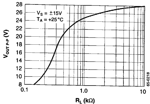
Figure 8. Output Voltage Swing vs. Load Resistance
