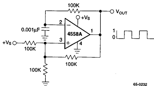
Figure 22. Squarewave Oscillator
