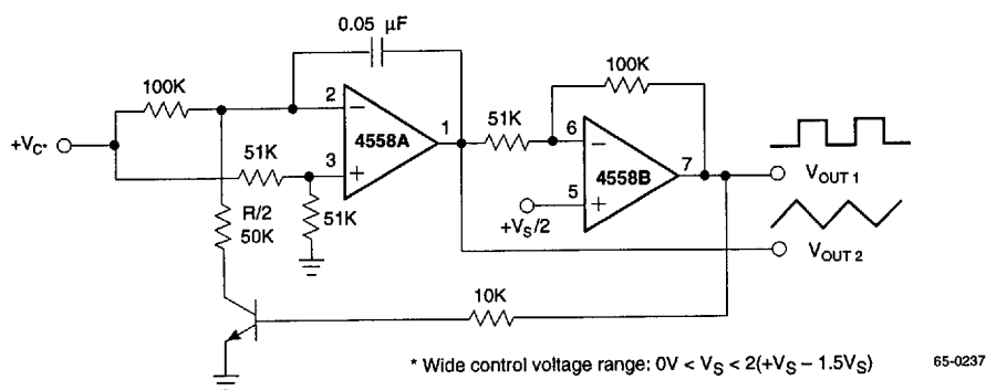
Figure 27. Voltage Controlled Oscillator (VCO)
