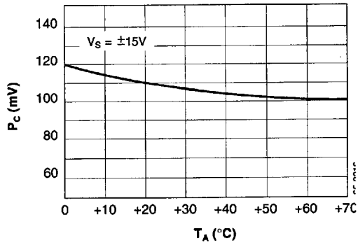
Figure 6. Power Consumption vs. Temperature
