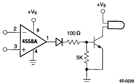
Figure 19. Lamp Driver
