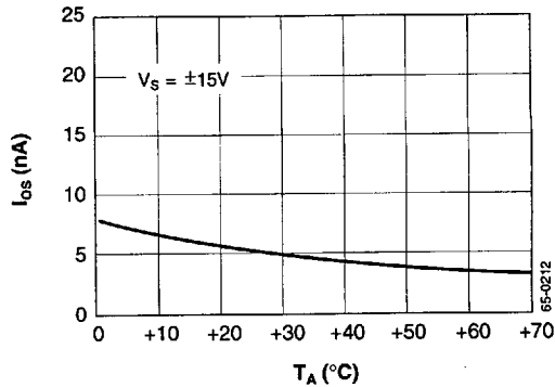
Figure 2. Input Offset Current vs. Temperature
