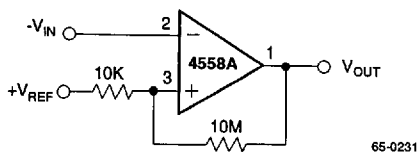
Figure 21. Comparator With Hysteresis
