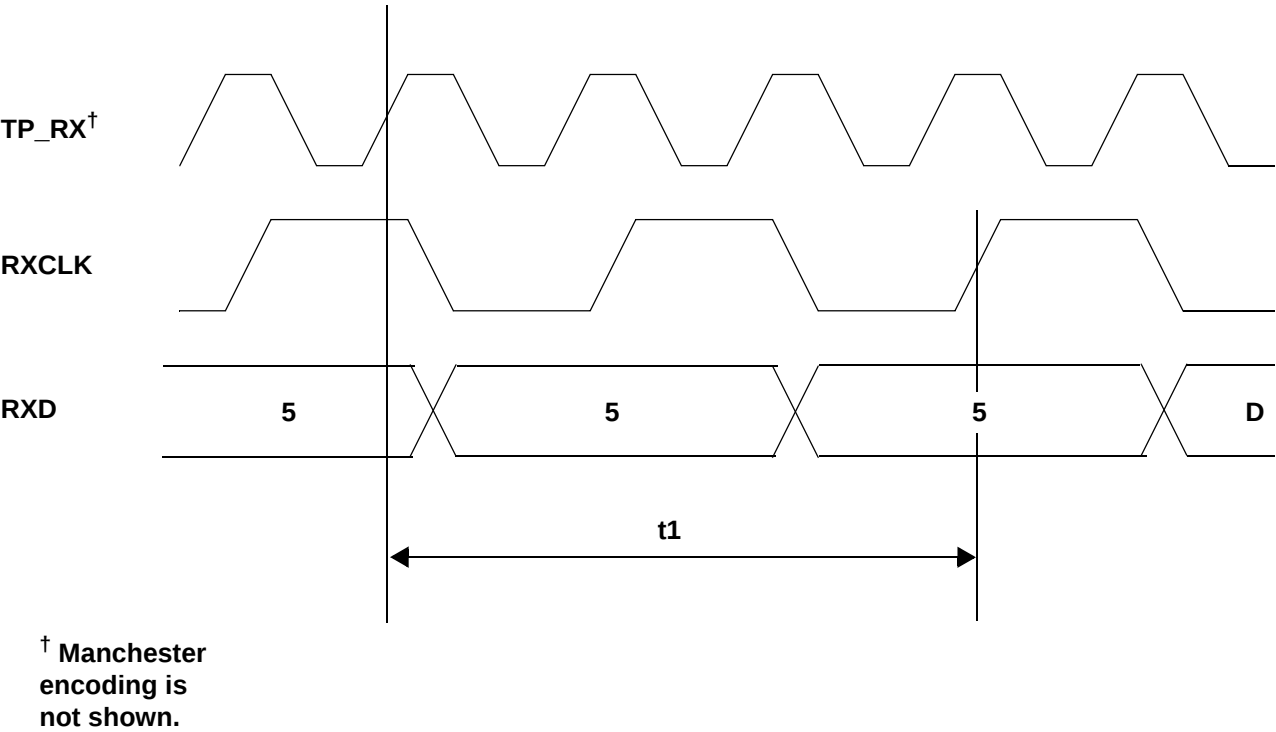
10M MII Receive Latency Timing Diagram
