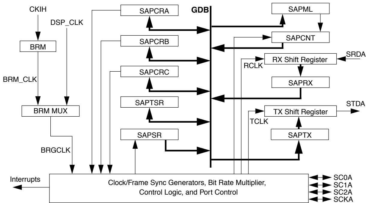
Figure 14-1. SAP Block Diagram
