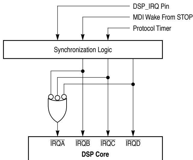
Figure 7-3. Internal \overline{\text{IRQA}}\text{--}\overline{\text{D}} Connection
