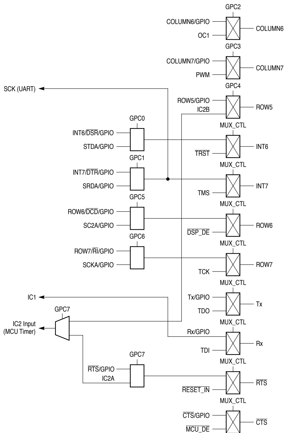
Figure 4-4. MUX Connectivity Scheme
