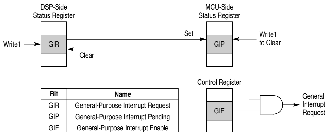
Figure 5-6. DSP-to-MCU General Purpose Interrupt
