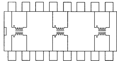
16-Pin Triple Schematic
