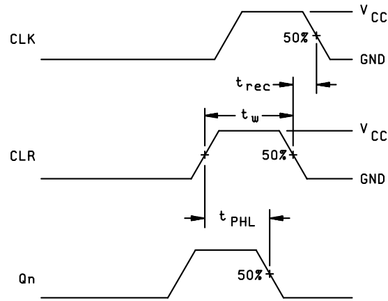
FIGURE 4. Switching waveforms and test circuit.
