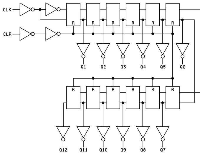
FIGURE 3. Logic diagram.
