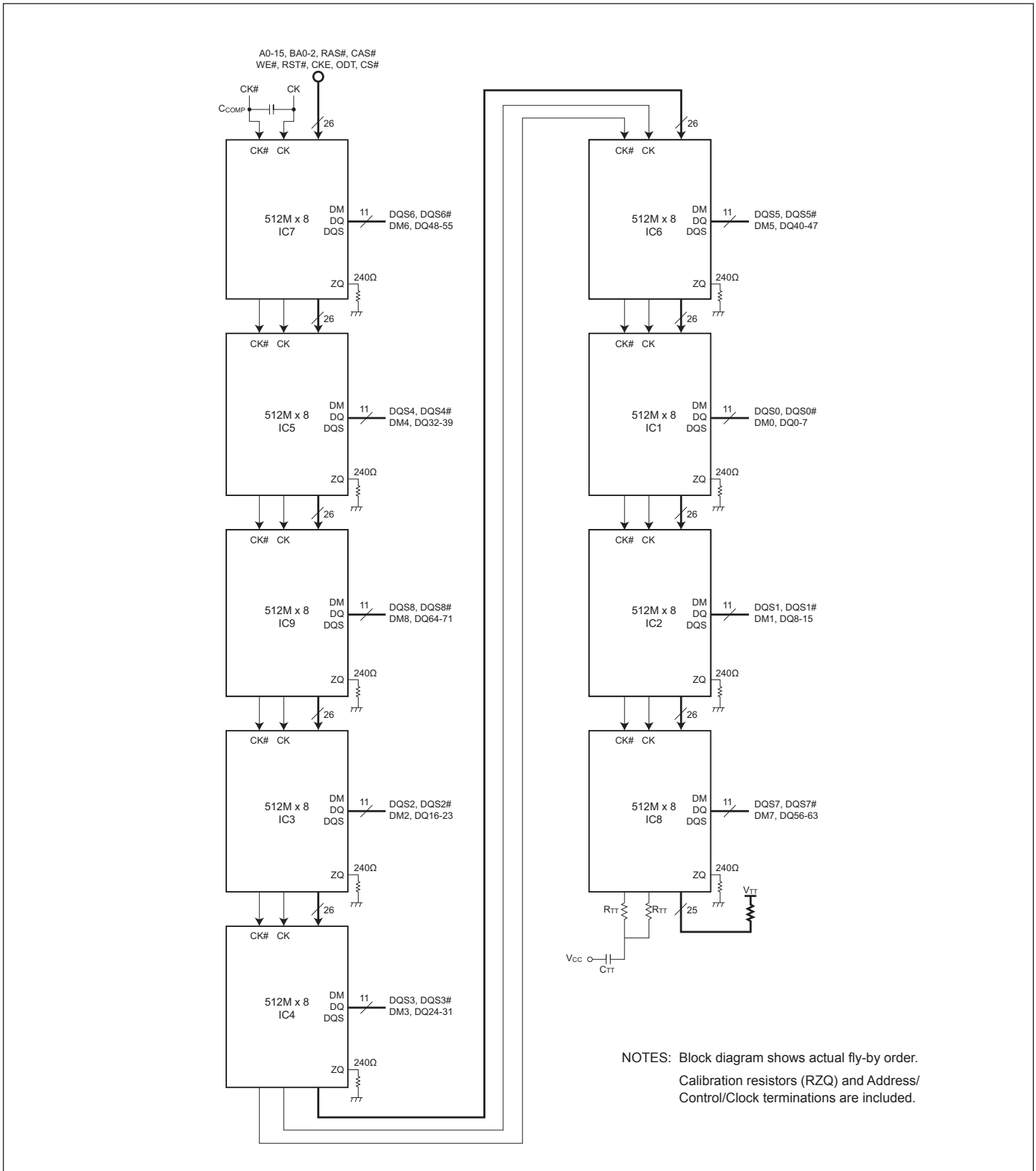
FIGURE 2 – FUNCTIONAL BLOCK DIAGRAM FOR W3J512M72G-XLBX
