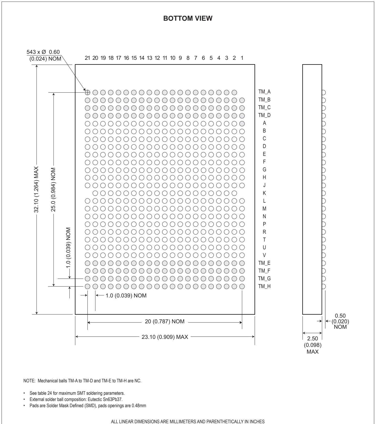
FIGURE 15 – PACKAGE DIMENSION: 543 PBGA, LOW PROFILE for W3J512M72G-XLBX
