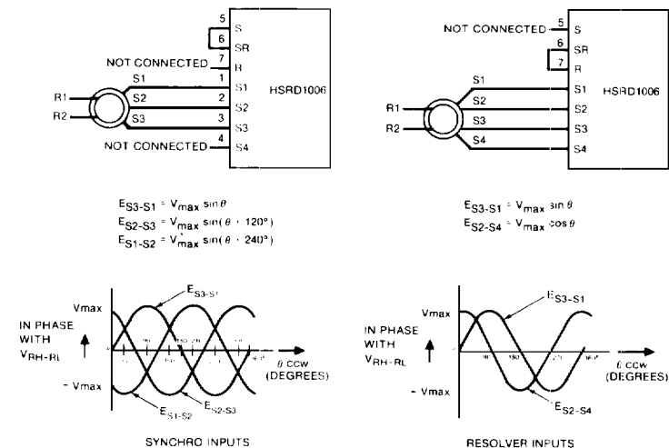
FIGURE 7 Synchro/Resolver Inputs
