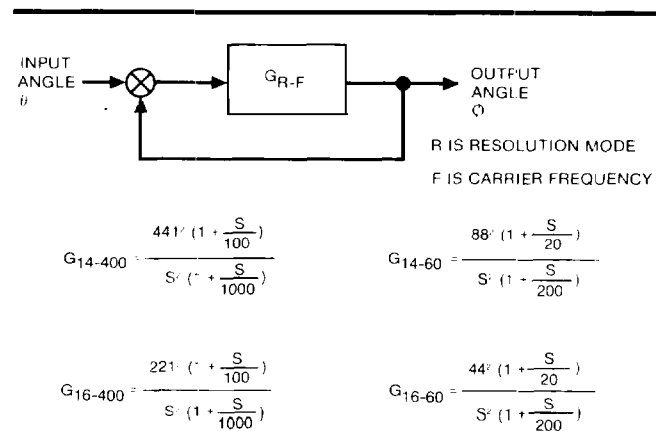
FIGURE 4 Transfer Functions for HSRD1006
