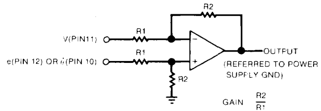
FIGURE 2 Difference Circuit for Bipolar Analog Outputs
