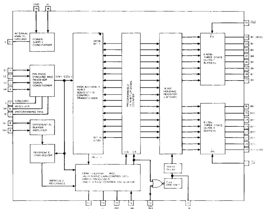
FIGURE 1 1006 Block Diagram
