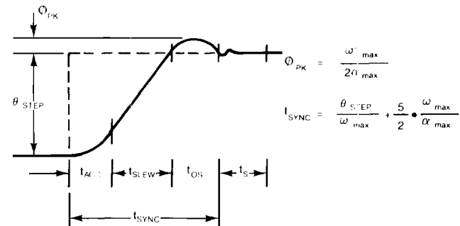
FIGURE 3 Large Signal ( \geq 1.4^\circ ) Response Parameters
